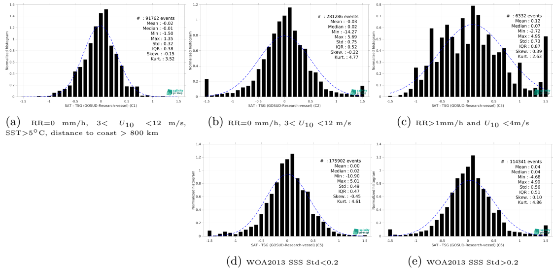
Figure 13: Normalized histogram of \Delta\text{SSS} (SMAP SSS L2 v5 (RSS) - TSG (GOSUD-Research-vessel)) for 5 different subdatasets corresponding to: RR=0 mm/h, 3 < U_{10} < 12 m/s, SST>5°C, distance to coast > 800 km (a), RR=0 mm/h, 3 < U_{10} < 12 m/s (b), RR>1mm/h and U_{10} < 4 m/s (c), WOA2013 SSS Std<0.2 (d), WOA2013 SSS Std>0.2 (e).
