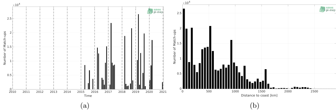
Figure 1: Number of match-ups between TSG (GOSUD-Research-vessel) and SMAP SSS L2 v5 (RSS) SSS as a function of time (a) and as function of the distance to coast (b) over the Equatorial Ocean 10N-10S Pi-MEP region and for the full satellite product period.
