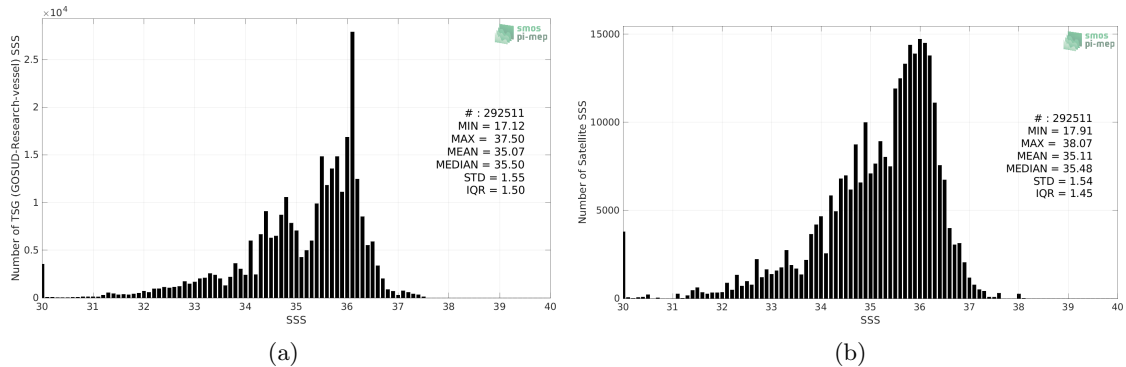
Figure 2: Histograms of SSS from TSG (GOSUD-Research-vessel) (a) and SMAP SSS L2 v5 (RSS) (b) considering all match-up pairs per bins of 0.1 over the Equatorial Ocean 10N-10S Pi-MEP region and for the full satellite product period.
