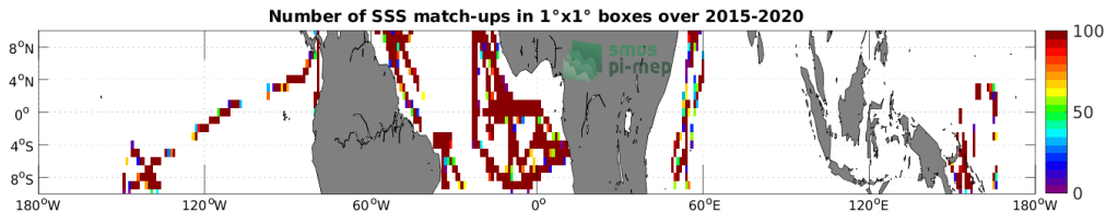
Figure 4: Number of SSS match-ups between TSG (GOSUD-Research-vessel) SSS and the SMAP SSS L2 v5 (RSS) SSS product for the Equatorial Ocean 10N-10S Pi-MEP region over 1^\circ \times 1^\circ boxes and for the full satellite product period.
