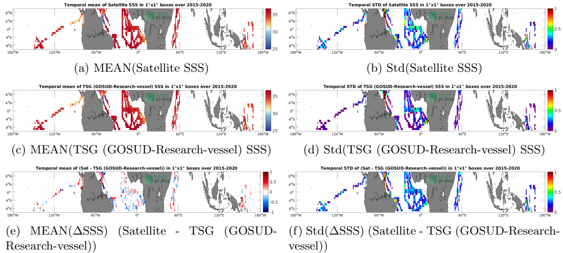
Figure 6: Temporal mean (left) and Std (right) of SSS from SMAP SSS L2 v5 (RSS) (top), TSG (GOSUD-Research-vessel) (middle), and of \Delta SSS (Satellite - TSG (GOSUD-Research-vessel)). Only match-up pairs are used to generate these maps.
