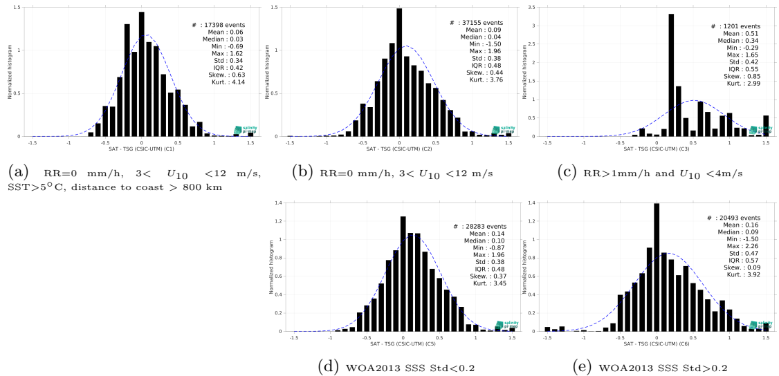
Figure 13: Normalized histogram of \Delta SSS (SMAP SSS L2 v5 (RSS) - TSG (CSIC-UTM)) for 5 different subdatasets corresponding to: RR=0 mm/h, 3 < U_{10} < 12 m/s, SST >5^\circ\text{C} , distance to coast > 800 km (a), RR=0 mm/h, 3 < U_{10} < 12 m/s (b), RR >1 mm/h and U_{10} < 4 m/s (c), WOA2013 SSS Std <0.2 (d), WOA2013 SSS Std >0.2 (e).
