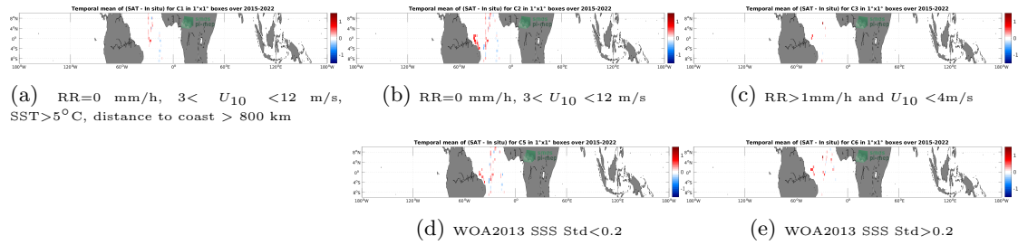
Figure 12: Temporal mean gridded over spatial boxes of size 1^\circ \times 1^\circ of \Delta SSS (SMAP SSS L2 v5 (RSS) - TSG (CSIC-UTM)) for 5 different subdatasets corresponding to:RR=0 mm/h, 3 < U_{10} < 12 m/s, SST >5^\circ\text{C} , distance to coast > 800 km (a), RR=0 mm/h, 3 < U_{10} < 12 m/s (b), RR >1 mm/h and U_{10} < 4 m/s (c), WOA2013 SSS Std <0.2 (d), WOA2013 SSS Std >0.2 (e).
