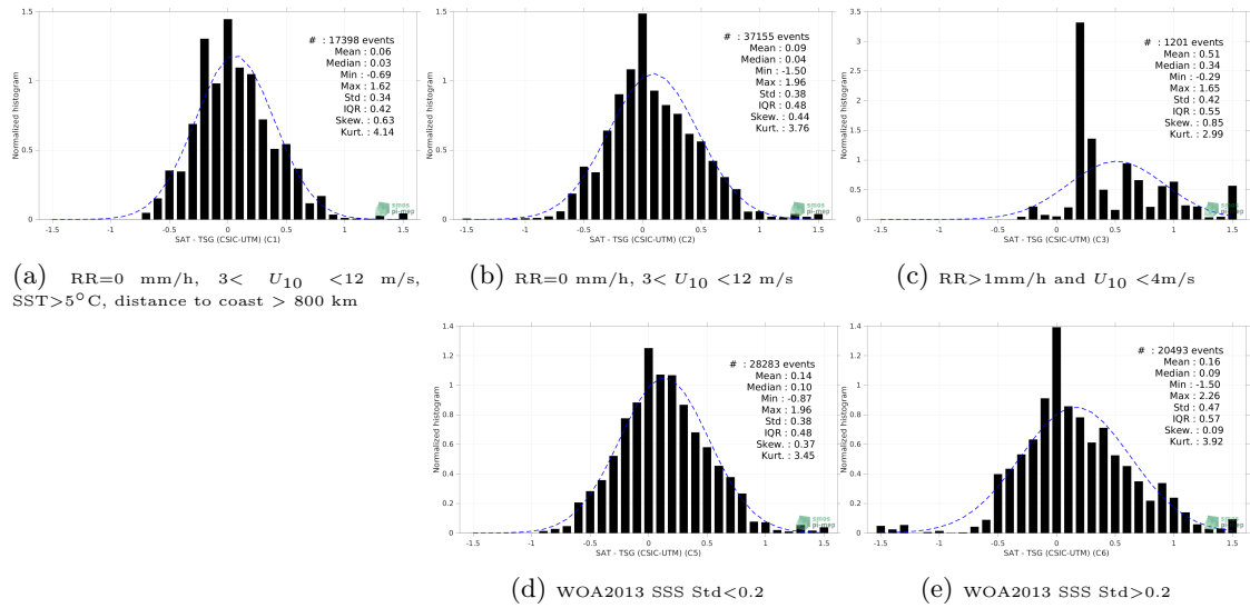
Figure 13: Normalized histogram of \Delta SSS (SMAP SSS L2 v5 (RSS) - TSG (CSIC-UTM)) for 5 different subdatasets corresponding to: RR=0 mm/h, 3 < U_{10} < 12 m/s, SST >5^\circ\text{C} , distance to coast > 800 km (a), RR=0 mm/h, 3 < U_{10} < 12 m/s (b), RR >1 mm/h and U_{10} < 4 m/s (c), WOA2013 SSS Std <0.2 (d), WOA2013 SSS Std >0.2 (e).
