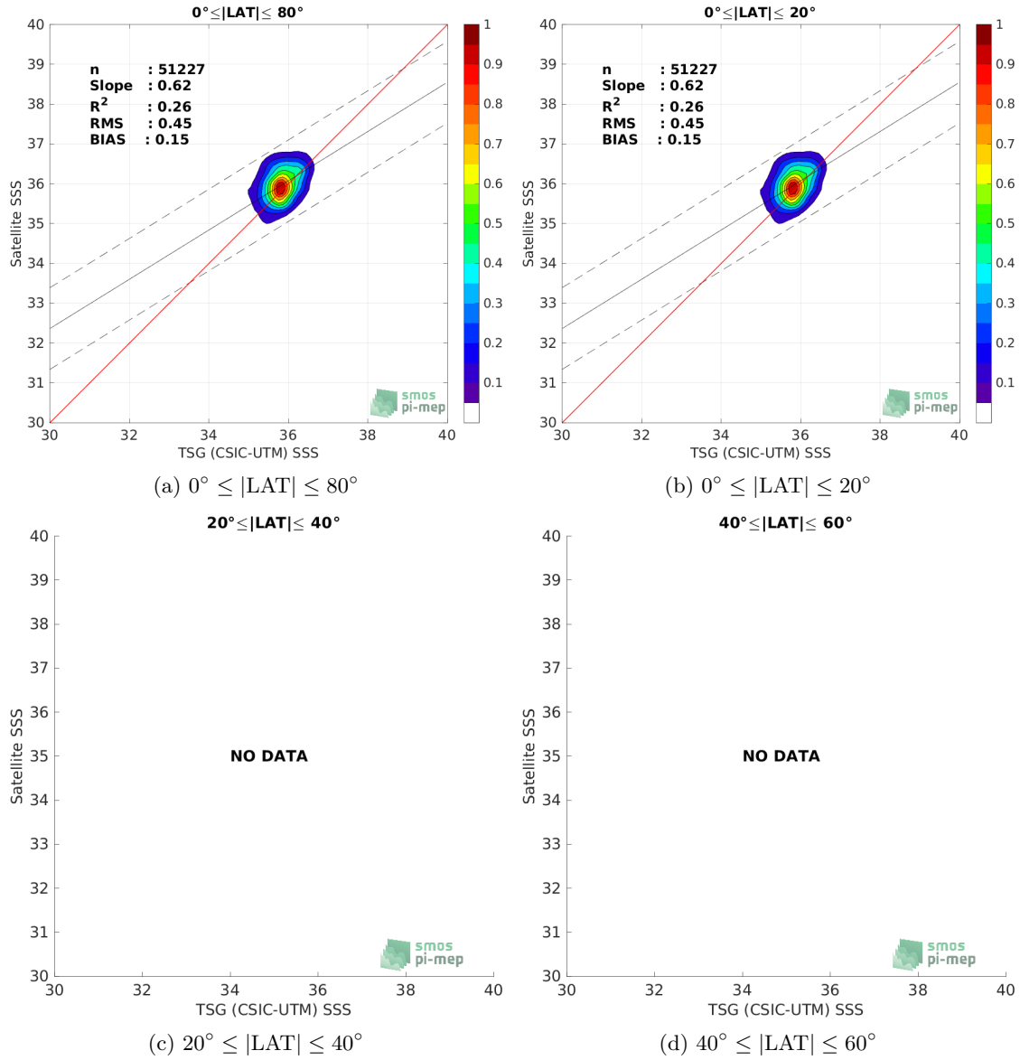
Figure 9: Contour maps of the concentration of SMAP SSS L2 v5 (RSS) SSS (y-axis) versus TSG (CSIC-UTM) SSS (x-axis) at match-up pairs for different latitude bands. For each plot, the red line shows x=y . The black thin and dashed lines indicate a linear fit through the data cloud and the \pm 95\% confidence levels, respectively. The number match-up pairs n , the slope and R^2 coefficient of the linear fit, the root mean square (RMS) and the mean bias between satellite and in situ data are indicated for each latitude band in each plots.
