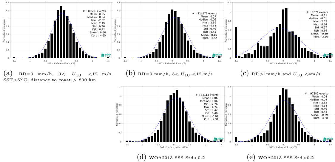
Figure 12: Normalized histogram of \Delta SSS (SMAP SSS L2 v5 (RSS) - Surface drifters) for 5 different subdatasets corresponding to: RR=0 mm/h, 3 < U_{10} < 12 m/s, SST >5^\circ C , distance to coast > 800 km (a), RR=0 mm/h, 3 < U_{10} < 12 m/s (b), RR >1 mm/h and U_{10} < 4 m/s (c), WOA2013 SSS Std <0.2 (d), WOA2013 SSS Std >0.2 (e).
