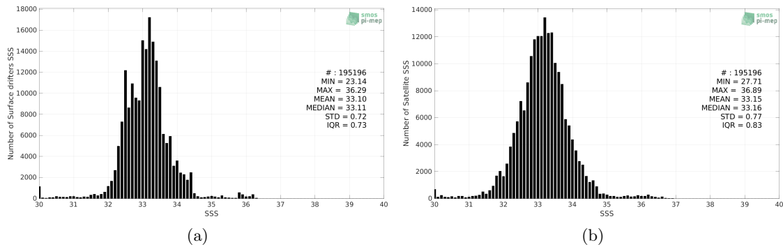
Figure 2: Histograms of SSS from Surface drifters (a) and SMAP SSS L2 v5 (RSS) (b) considering all match-up pairs per bins of 0.1 over the Equatorial Ocean 10N-10S Pi-MEP region and for the full satellite product period.
