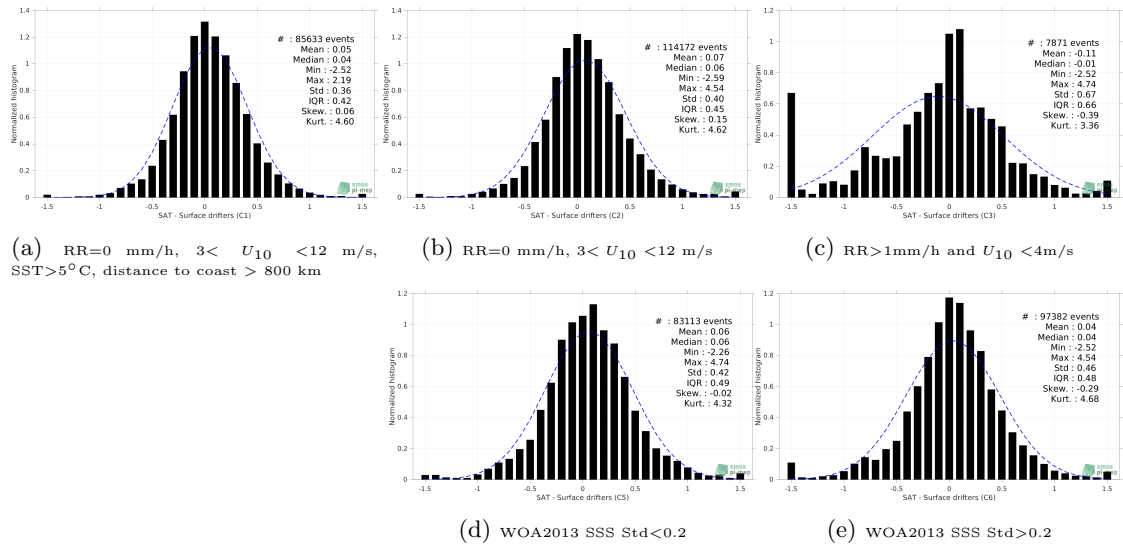
Figure 12: Normalized histogram of \Delta SSS (SMAP SSS L2 v5 (RSS) - Surface drifters) for 5 different subdatasets corresponding to: RR=0 mm/h, 3 < U_{10} < 12 m/s, SST >5^\circ\text{C} , distance to coast > 800 km (a), RR=0 mm/h, 3 < U_{10} < 12 m/s (b), RR >1 mm/h and U_{10} < 4 m/s (c), WOA2013 SSS Std <0.2 (d), WOA2013 SSS Std >0.2 (e).
