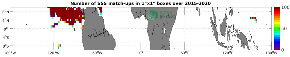
Figure 3: Number of SSS match-ups between Surface drifters SSS and the SMAP SSS L2 v5 (RSS) SSS product for the Equatorial Ocean 10N-10S Pi-MEP region over 1^\circ \times 1^\circ boxes and for the full satellite product period.
