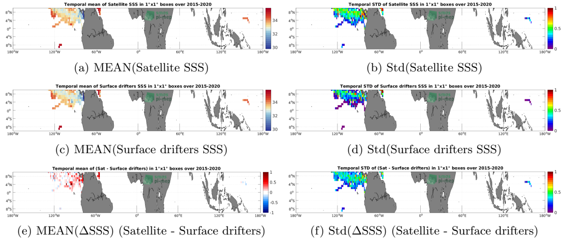
Figure 5: Temporal mean (left) and Std (right) of SSS from SMAP SSS L2 v5 (RSS) (top), Surface drifters (middle), and of \Delta SSS (Satellite - Surface drifters). Only match-up pairs are used to generate these maps.
