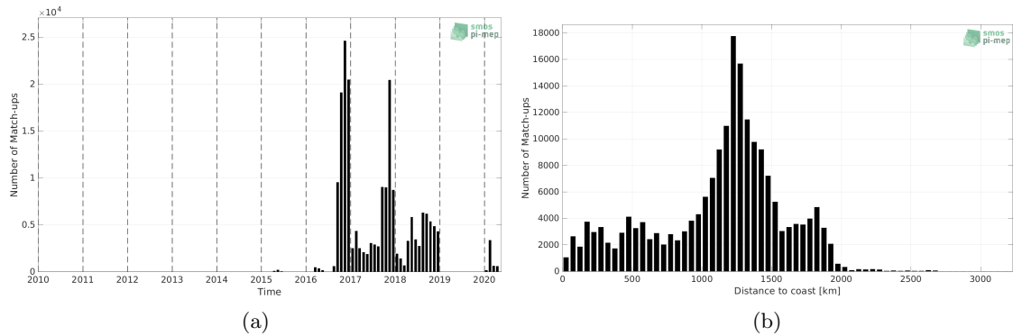
Figure 1: Number of match-ups between Surface drifters and SMAP SSS L2 v5 (RSS) SSS as a function of time (a) and as function of the distance to coast (b) over the Equatorial Ocean 10N-10S Pi-MEP region and for the full satellite product period.
