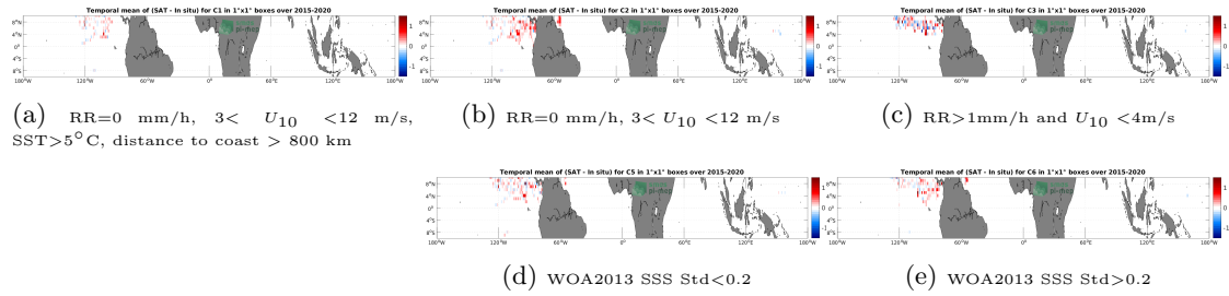
Figure 11: Temporal mean gridded over spatial boxes of size 1^\circ \times 1^\circ of \Delta SSS (SMAP SSS L2 v5 (RSS) - Surface drifters) for 5 different subdatasets corresponding to:RR=0 mm/h, 3 < U_{10} < 12 m/s, SST >5^\circ\text{C} , distance to coast > 800 km (a), RR=0 mm/h, 3 < U_{10} < 12 m/s (b), RR >1 mm/h and U_{10} < 4 m/s (c), WOA2013 SSS Std <0.2 (d), WOA2013 SSS Std >0.2 (e).
