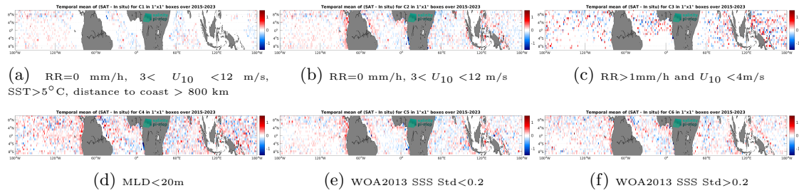
Figure 12: Temporal mean gridded over spatial boxes of size 1^\circ \times 1^\circ of \Delta SSS (SMAP SSS L2 v5 (RSS) - Argo) for 6 different subdatasets corresponding to: RR=0 mm/h, 3 < U_{10} < 12 m/s, SST > 5^\circ\text{C} , distance to coast > 800 km (a), RR=0 mm/h, 3 < U_{10} < 12 m/s (b), RR > 1 mm/h and U_{10} < 4 m/s (c), MLD < 20 m (d), WOA2013 SSS Std < 0.2 (e), WOA2013 SSS Std > 0.2 (f).
