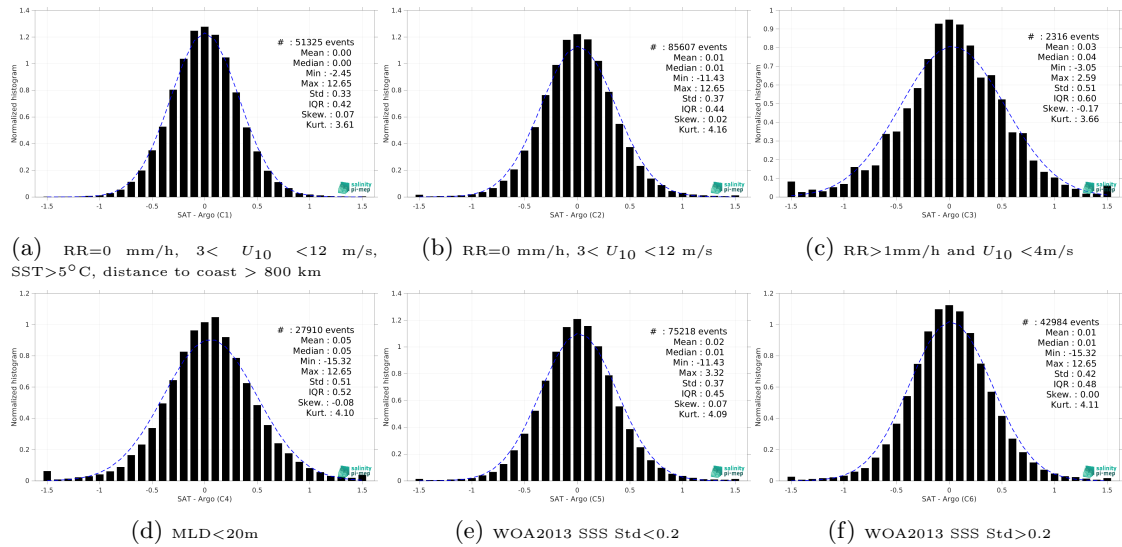
Figure 13: Normalized histogram of \Delta SSS (SMAP SSS L2 v5 (RSS) - Argo) for 6 different subdatasets corresponding to: RR=0 mm/h, 3 < U_{10} < 12 m/s, SST > 5^\circ\text{C} , distance to coast > 800 km (a), RR=0 mm/h, 3 < U_{10} < 12 m/s (b), RR > 1 mm/h and U_{10} < 4 m/s (c), MLD < 20 m (d), WOA2013 SSS Std < 0.2 (e), WOA2013 SSS Std > 0.2 (f).
