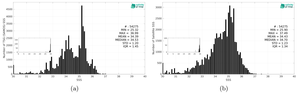
Figure 3: Histograms of SSS from TSG (SAMOS) (a) and SMAP SSS L2 v5.3 (RSS) (b) considering all match-up pairs per bins of 0.1 over the Equatorial Ocean 10N-10S Pi-MEP region and for the full satellite product period.
