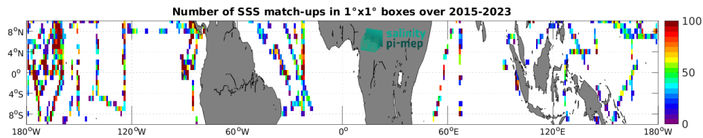
Figure 5: Number of SSS match-ups between TSG (SAMOS) SSS and the SMAP SSS L2 v5.3 (RSS) SSS product for the Equatorial Ocean 10N-10S Pi-MEP region over 1^\circ \times 1^\circ boxes and for the full satellite product period.
