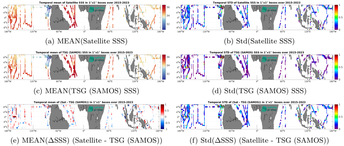
Figure 7: Temporal mean (left) and Std (right) of SSS from SMAP SSS L2 v5.3 (RSS) (top), TSG (SAMOS) (middle), and of \Delta SSS (Satellite - TSG (SAMOS)). Only match-up pairs are used to generate these maps.
