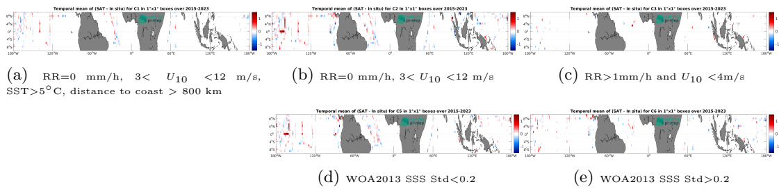
Figure 14: Temporal mean gridded over spatial boxes of size 1^\circ \times 1^\circ of \Delta SSS (SMAP SSS L2 v5.3 (RSS) - TSG (SAMOS)) for 5 different subdatasets corresponding to:RR=0 mm/h, 3 < U_{10} < 12 m/s, SST>5°C, distance to coast > 800 km (a), RR=0 mm/h, 3 < U_{10} < 12 m/s (b), RR>1mm/h and U_{10} < 4 m/s (c), WOA2013 SSS Std<0.2 (d), WOA2013 SSS Std>0.2 (e).
