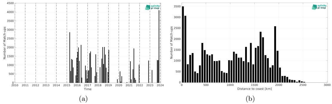
Figure 2: Number of match-ups between TSG (SAMOS) and SMAP SSS L2 v5.3 (RSS) SSS as a function of time (a) and as function of the distance to coast (b) over the Equatorial Ocean 10N-10S Pi-MEP region and for the full satellite product period.
