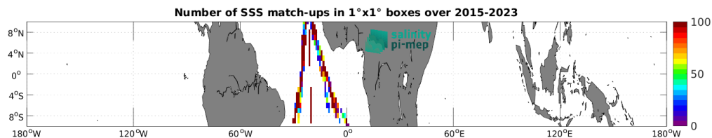
Figure 5: Number of SSS match-ups between TSG (Polarstern) SSS and the SMAP SSS L2 v5.3 (RSS) SSS product for the Equatorial Ocean 10N-10S Pi-MEP region over 1^\circ \times 1^\circ boxes and for the full satellite product period.
