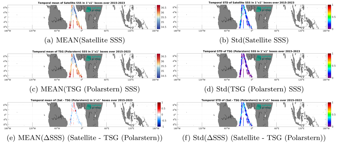
Figure 7: Temporal mean (left) and Std (right) of SSS from SMAP SSS L2 v5.3 (RSS) (top), TSG (Polarstern) (middle), and of \Delta SSS (Satellite - TSG (Polarstern)). Only match-up pairs are used to generate these maps.
