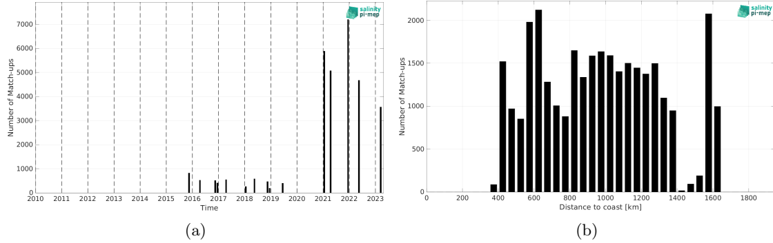
Figure 2: Number of match-ups between TSG (Polarstern) and SMAP SSS L2 v5.3 (RSS) SSS as a function of time (a) and as function of the distance to coast (b) over the Equatorial Ocean 10N-10S Pi-MEP region and for the full satellite product period.
