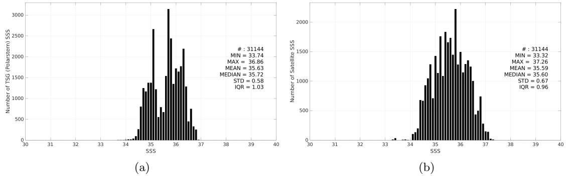
Figure 3: Histograms of SSS from TSG (Polarstern) (a) and SMAP SSS L2 v5.3 (RSS) (b) considering all match-up pairs per bins of 0.1 over the Equatorial Ocean 10N-10S Pi-MEP region and for the full satellite product period.
