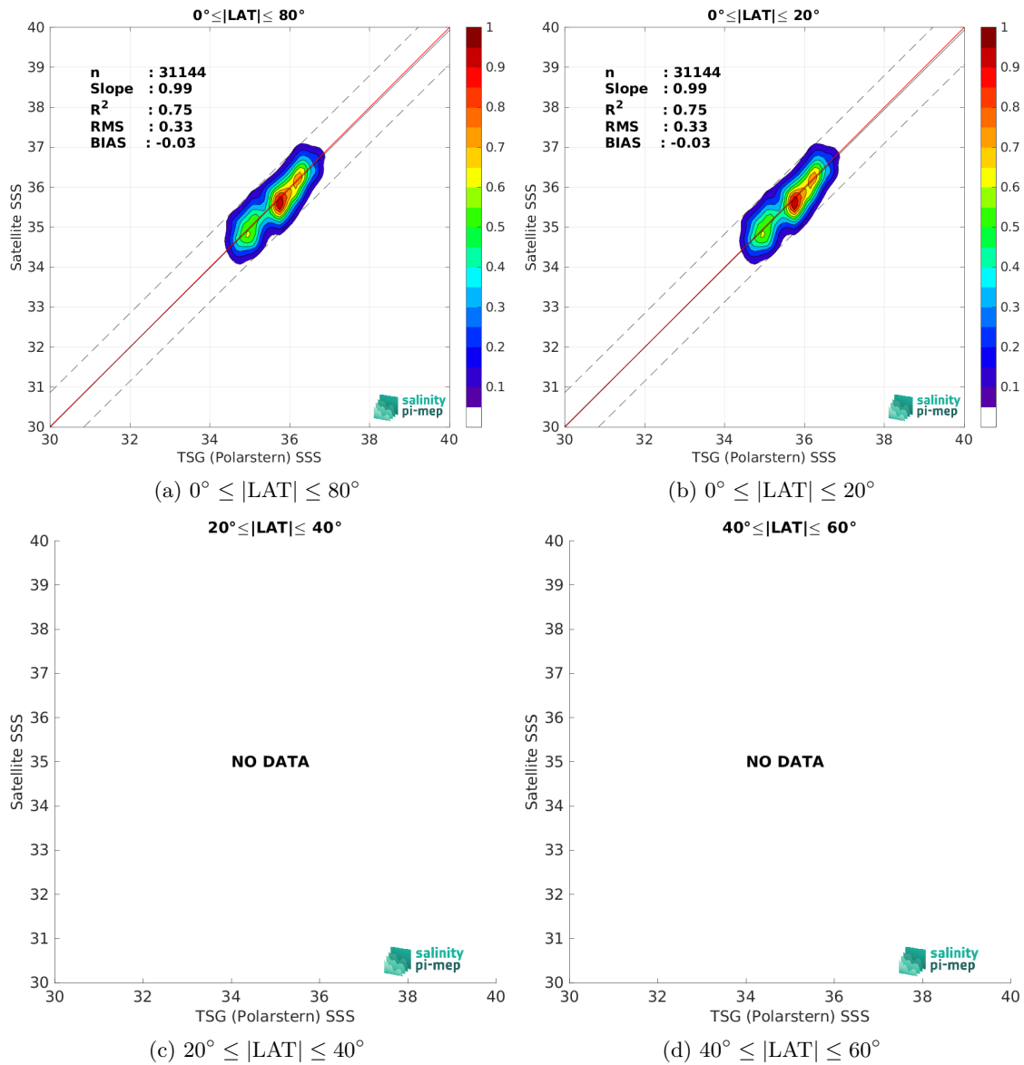
Figure 10: Contour maps of the concentration of SMAP SSS L2 v5.3 (RSS) SSS (y-axis) versus TSG (Polarstern) SSS (x-axis) at match-up pairs for different latitude bands. For each plot, the red line shows x=y . The black thin and dashed lines indicate a linear fit through the data cloud and the \pm 95\% confidence levels, respectively. The number match-up pairs n , the slope and R^2 coefficient of the linear fit, the root mean square (RMS) and the mean bias between satellite and in situ data are indicated for each latitude band in each plots.
