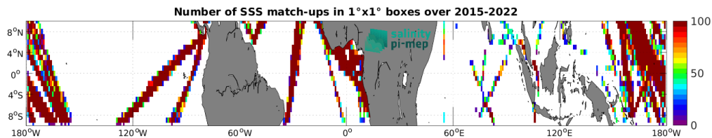
Figure 5: Number of SSS match-ups between TSG (LEGOS-DM) SSS and the SMAP SSS L2 v5.3 (RSS) SSS product for the Equatorial Ocean 10N-10S Pi-MEP region over 1^\circ \times 1^\circ boxes and for the full satellite product period.
