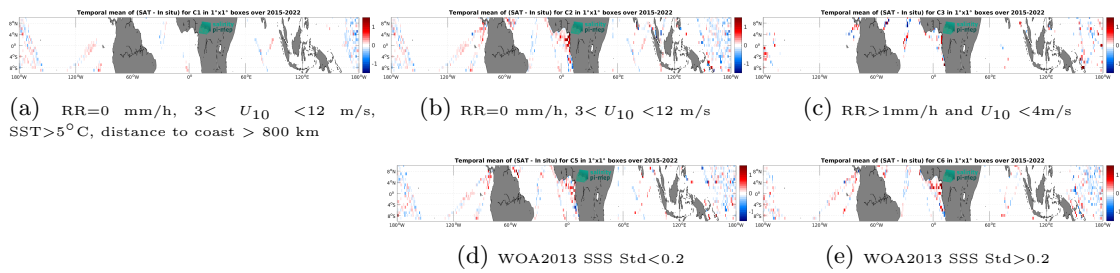
Figure 14: Temporal mean gridded over spatial boxes of size 1^\circ \times 1^\circ of \Delta SSS (SMAP SSS L2 v5.3 (RSS) - TSG (LEGOS-DM)) for 5 different subdatasets corresponding to:RR=0 mm/h, 3 < U_{10} < 12 m/s, SST>5°C, distance to coast > 800 km (a), RR=0 mm/h, 3 < U_{10} < 12 m/s (b), RR>1mm/h and U_{10} < 4 m/s (c), WOA2013 SSS Std<0.2 (d), WOA2013 SSS Std>0.2 (e).
