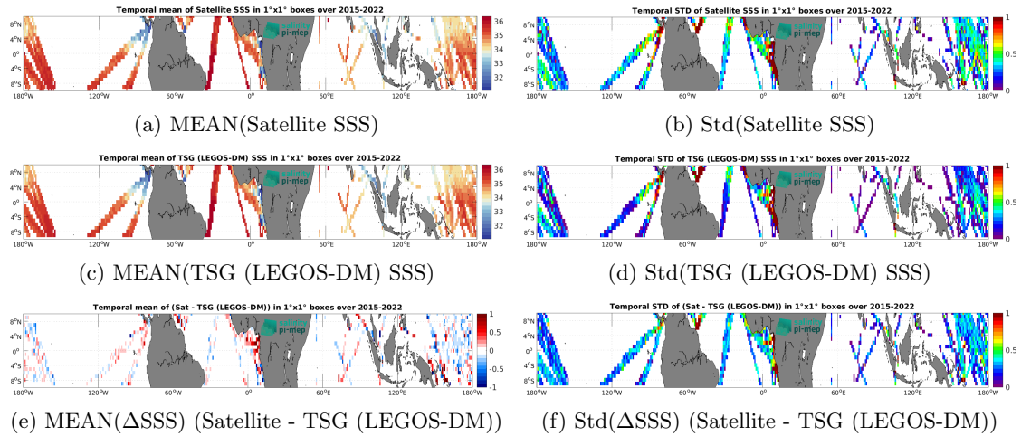
Figure 7: Temporal mean (left) and Std (right) of SSS from SMAP SSS L2 v5.3 (RSS) (top), TSG (LEGOS-DM) (middle), and of \Delta SSS (Satellite - TSG (LEGOS-DM)). Only match-up pairs are used to generate these maps.
