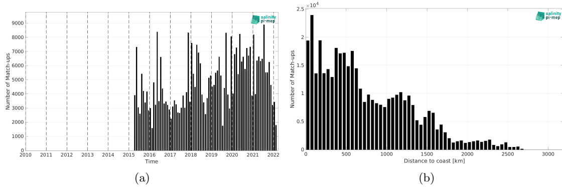
Figure 2: Number of match-ups between TSG (LEGOS-DM) and SMAP SSS L2 v5.3 (RSS) SSS as a function of time (a) and as function of the distance to coast (b) over the Equatorial Ocean 10N-10S Pi-MEP region and for the full satellite product period.
