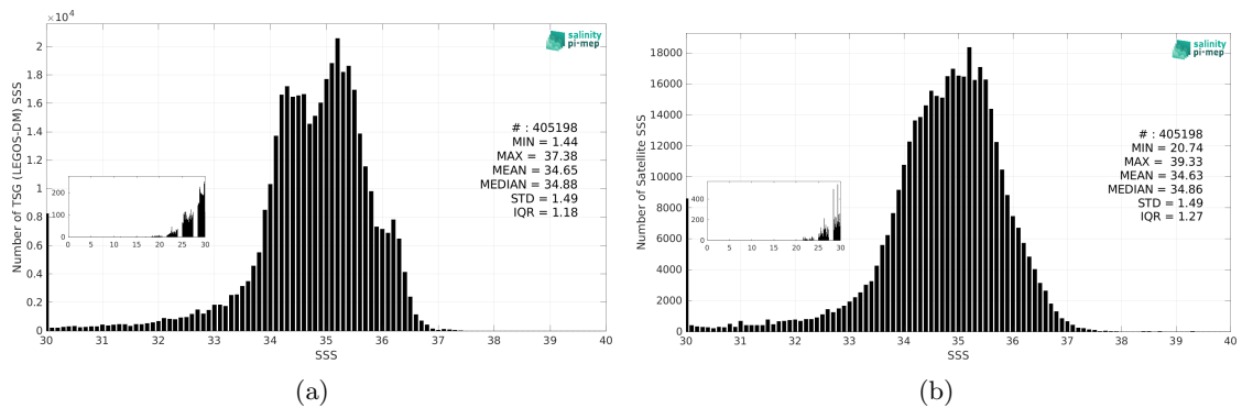
Figure 3: Histograms of SSS from TSG (LEGOS-DM) (a) and SMAP SSS L2 v5.3 (RSS) (b) considering all match-up pairs per bins of 0.1 over the Equatorial Ocean 10N-10S Pi-MEP region and for the full satellite product period.
