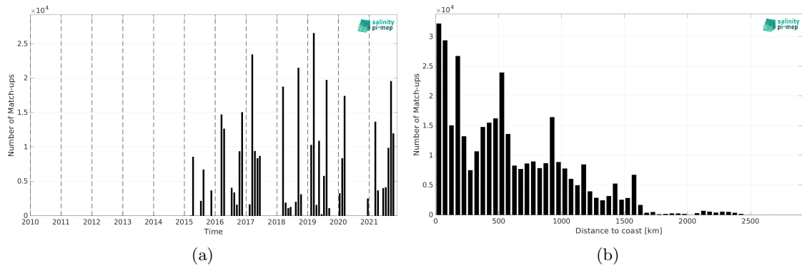
Figure 2: Number of match-ups between TSG (GOSUD-Research-vessel) and SMAP SSS L2 v5.3 (RSS) SSS as a function of time (a) and as function of the distance to coast (b) over the Equatorial Ocean 10N-10S Pi-MEP region and for the full satellite product period.
