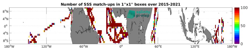
Figure 5: Number of SSS match-ups between TSG (GOSUD-Research-vessel) SSS and the SMAP SSS L2 v5.3 (RSS) SSS product for the Equatorial Ocean 10N-10S Pi-MEP region over 1^\circ \times 1^\circ boxes and for the full satellite product period.
