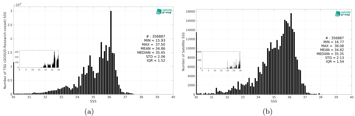
Figure 3: Histograms of SSS from TSG (GOSUD-Research-vessel) (a) and SMAP SSS L2 v5.3 (RSS) (b) considering all match-up pairs per bins of 0.1 over the Equatorial Ocean 10N-10S Pi-MEP region and for the full satellite product period.
