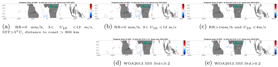
Figure 14: Temporal mean gridded over spatial boxes of size 1^\circ \times 1^\circ of \Delta SSS (SMAP SSS L2 v5.3 (RSS) - TSG (GOSUD-Research-vessel)) for 5 different subdatasets corresponding to: RR=0 mm/h, 3 < U_{10} < 12 m/s, SST>5°C, distance to coast > 800 km (a), RR=0 mm/h, 3 < U_{10} < 12 m/s (b), RR>1mm/h and U_{10} < 4 m/s (c), WOA2013 SSS Std<0.2 (d), WOA2013 SSS Std>0.2 (e).
