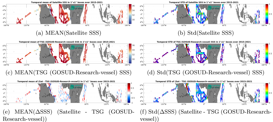
Figure 7: Temporal mean (left) and Std (right) of SSS from SMAP SSS L2 v5.3 (RSS) (top), TSG (GOSUD-Research-vessel) (middle), and of \Delta SSS (Satellite - TSG (GOSUD-Research-vessel)). Only match-up pairs are used to generate these maps.
