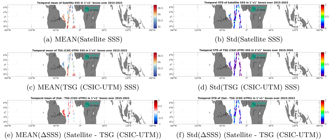
Figure 7: Temporal mean (left) and Std (right) of SSS from SMAP SSS L2 v5.3 (RSS) (top), TSG (CSIC-UTM) (middle), and of \Delta SSS (Satellite - TSG (CSIC-UTM)). Only match-up pairs are used to generate these maps.
