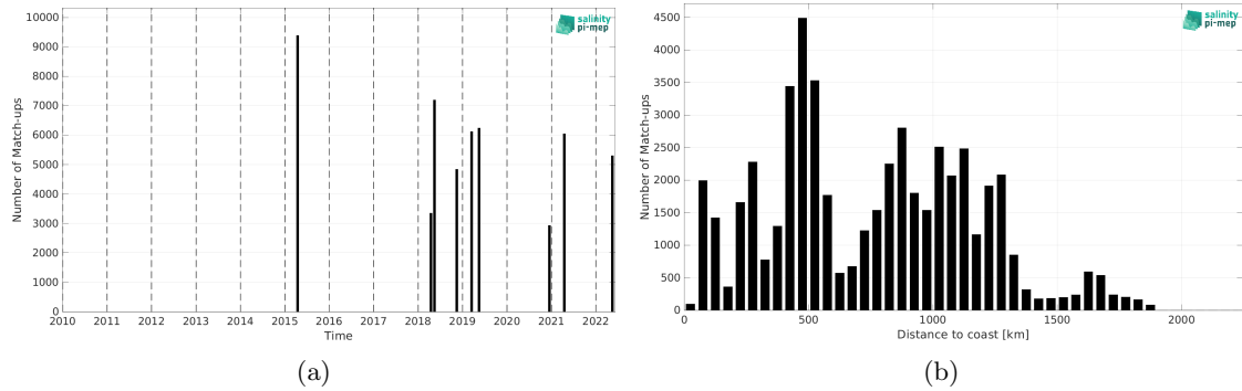
Figure 2: Number of match-ups between TSG (CSIC-UTM) and SMAP SSS L2 v5.3 (RSS) SSS as a function of time (a) and as function of the distance to coast (b) over the Equatorial Ocean 10N-10S Pi-MEP region and for the full satellite product period.
