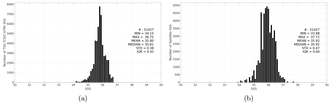
Figure 3: Histograms of SSS from TSG (CSIC-UTM) (a) and SMAP SSS L2 v5.3 (RSS) (b) considering all match-up pairs per bins of 0.1 over the Equatorial Ocean 10N-10S Pi-MEP region and for the full satellite product period.
