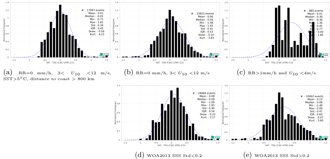
Figure 15: Normalized histogram of \Delta\text{SSS} (SMAP SSS L2 v5.3 (RSS) - TSG (CSIC-UTM)) for 5 different subdatasets corresponding to: RR=0 mm/h, 3 < U_{10} < 12 m/s, SST>5°C, distance to coast > 800 km (a), RR=0 mm/h, 3 < U_{10} < 12 m/s (b), RR>1mm/h and U_{10} < 4 m/s (c), WOA2013 SSS Std<0.2 (d), WOA2013 SSS Std>0.2 (e).
