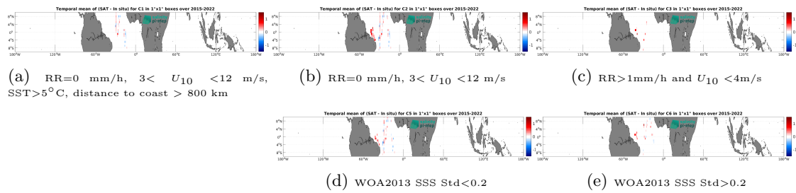
Figure 14: Temporal mean gridded over spatial boxes of size 1^\circ \times 1^\circ of \Delta\text{SSS} (SMAP SSS L2 v5.3 (RSS) - TSG (CSIC-UTM)) for 5 different subdatasets corresponding to:RR=0 mm/h, 3 < U_{10} < 12 m/s, SST>5°C, distance to coast > 800 km (a), RR=0 mm/h, 3 < U_{10} < 12 m/s (b), RR>1mm/h and U_{10} < 4 m/s (c), WOA2013 SSS Std<0.2 (d), WOA2013 SSS Std>0.2 (e).
