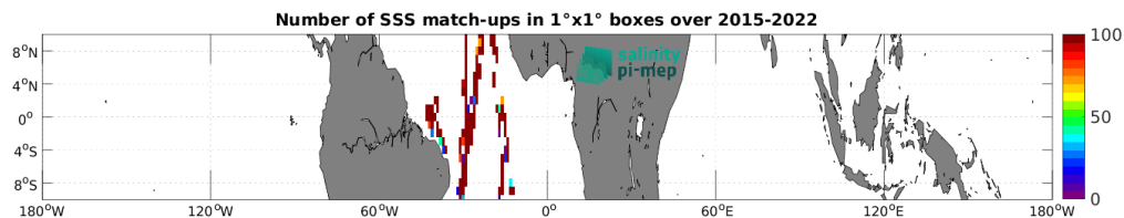
Figure 5: Number of SSS match-ups between TSG (CSIC-UTM) SSS and the SMAP SSS L2 v5.3 (RSS) SSS product for the Equatorial Ocean 10N-10S Pi-MEP region over 1^\circ \times 1^\circ boxes and for the full satellite product period.
