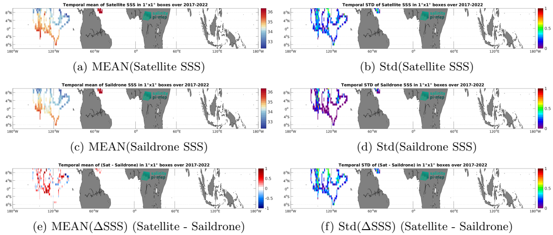
Figure 7: Temporal mean (left) and Std (right) of SSS from SMAP SSS L2 v5.3 (RSS) (top), Saildrone (middle), and of \Delta SSS (Satellite - Saildrone). Only match-up pairs are used to generate these maps.
