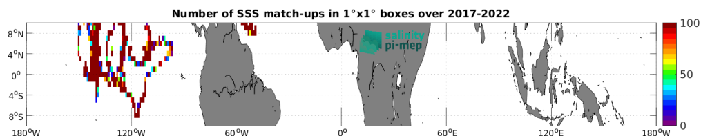
Figure 5: Number of SSS match-ups between Saildrone SSS and the SMAP SSS L2 v5.3 (RSS) SSS product for the Equatorial Ocean 10N-10S Pi-MEP region over 1^\circ \times 1^\circ boxes and for the full satellite product period.
