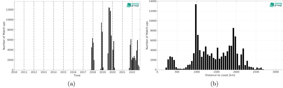
Figure 2: Number of match-ups between Saildrone and SMAP SSS L2 v5.3 (RSS) SSS as a function of time (a) and as function of the distance to coast (b) over the Equatorial Ocean 10N-10S Pi-MEP region and for the full satellite product period.
