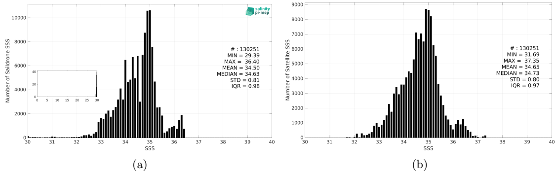
Figure 3: Histograms of SSS from Saildrone (a) and SMAP SSS L2 v5.3 (RSS) (b) considering all match-up pairs per bins of 0.1 over the Equatorial Ocean 10N-10S Pi-MEP region and for the full satellite product period.
