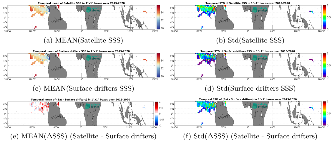
Figure 6: Temporal mean (left) and Std (right) of SSS from SMAP SSS L2 v5.3 (RSS) (top), Surface drifters (middle), and of \Delta SSS (Satellite - Surface drifters). Only match-up pairs are used to generate these maps.
