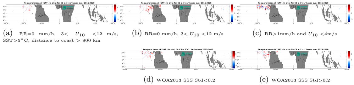
Figure 13: Temporal mean gridded over spatial boxes of size 1^\circ \times 1^\circ of \Delta SSS (SMAP SSS L2 v5.3 (RSS) - Surface drifters) for 5 different subdatasets corresponding to:RR=0 mm/h, 3 < U_{10} < 12 m/s, SST>5°C, distance to coast > 800 km (a), RR=0 mm/h, 3 < U_{10} < 12 m/s (b), RR>1mm/h and U_{10} < 4 m/s (c), WOA2013 SSS Std<0.2 (d), WOA2013 SSS Std>0.2 (e).
