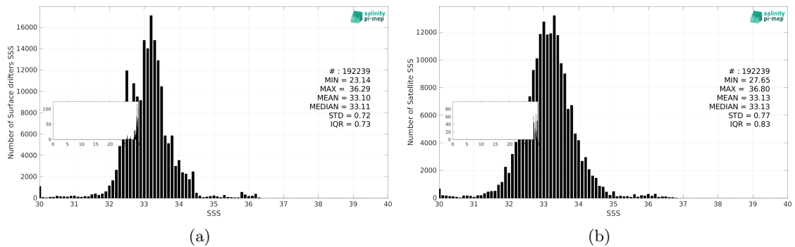
Figure 3: Histograms of SSS from Surface drifters (a) and SMAP SSS L2 v5.3 (RSS) (b) considering all match-up pairs per bins of 0.1 over the Equatorial Ocean 10N-10S Pi-MEP region and for the full satellite product period.
