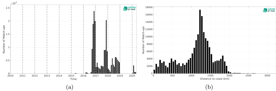
Figure 2: Number of match-ups between Surface drifters and SMAP SSS L2 v5.3 (RSS) SSS as a function of time (a) and as function of the distance to coast (b) over the Equatorial Ocean 10N-10S Pi-MEP region and for the full satellite product period.
