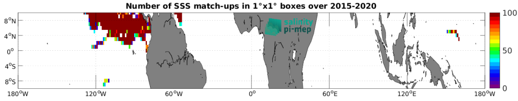
Figure 4: Number of SSS match-ups between Surface drifters SSS and the SMAP SSS L2 v5.3 (RSS) SSS product for the Equatorial Ocean 10N-10S Pi-MEP region over 1^\circ \times 1^\circ boxes and for the full satellite product period.
