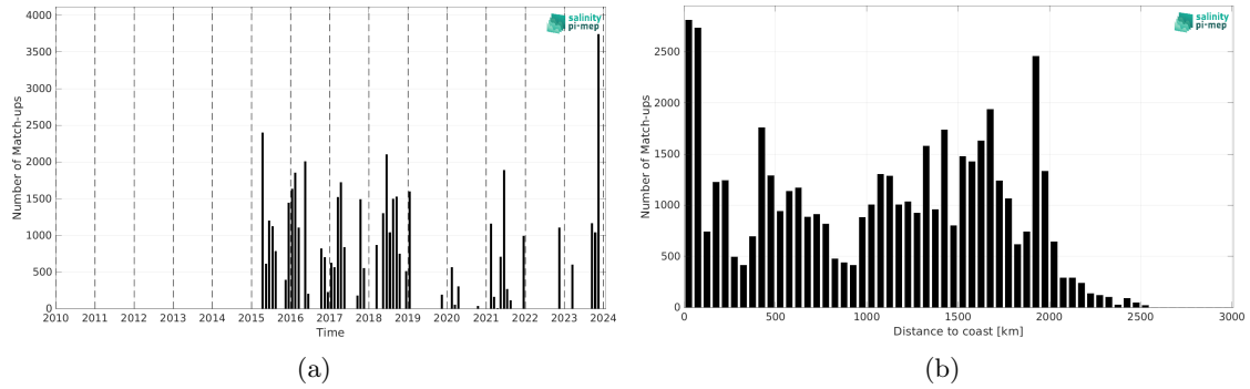
Figure 2: Number of match-ups between TSG (SAMOS) and SMAP SSS L2 v5.3 - 40 km (RSS) SSS as a function of time (a) and as function of the distance to coast (b) over the Equatorial Ocean 10N-10S Pi-MEP region and for the full satellite product period.
