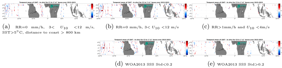
Figure 14: Temporal mean gridded over spatial boxes of size 1^\circ \times 1^\circ of \Delta SSS (SMAP SSS L2 v5.3 - 40 km (RSS) - TSG (SAMOS)) for 5 different subdatasets corresponding to:RR=0 mm/h, 3 < U_{10} < 12 m/s, SST>5°C, distance to coast > 800 km (a), RR=0 mm/h, 3 < U_{10} < 12 m/s (b), RR>1mm/h and U_{10} < 4 m/s (c), WOA2013 SSS Std<0.2 (d), WOA2013 SSS Std>0.2 (e).
