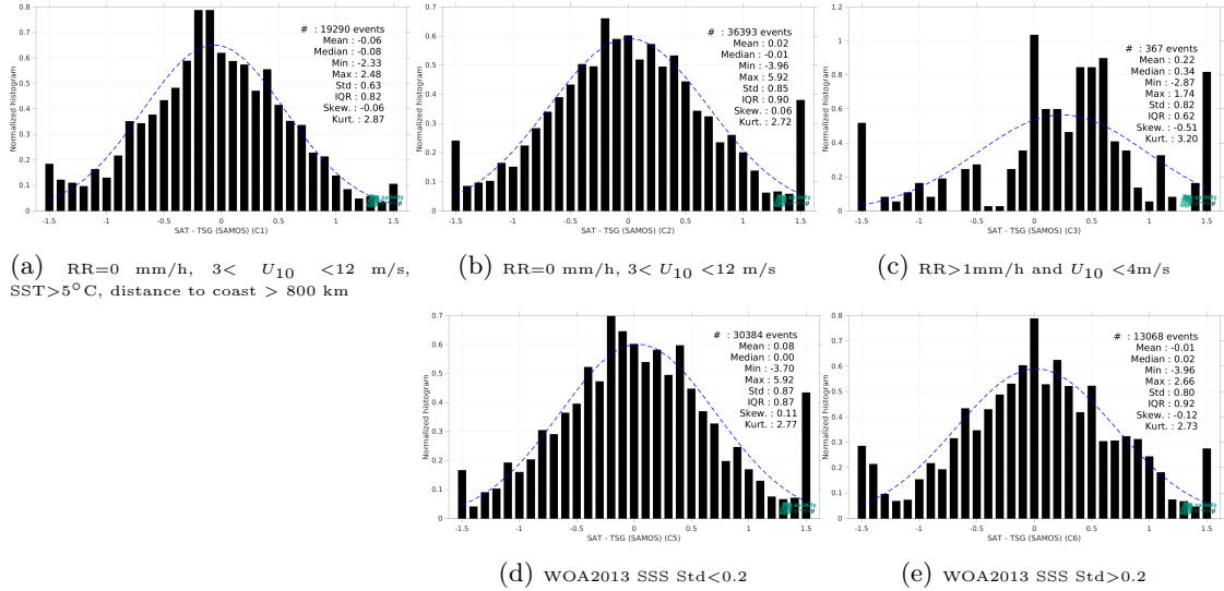
Figure 15: Normalized histogram of \Delta SSS (SMAP SSS L2 v5.3 - 40 km (RSS) - TSG (SAMOS)) for 5 different subdatasets corresponding to: RR=0 mm/h, 3 < U_{10} < 12 m/s, SST>5°C, distance to coast > 800 km (a), RR=0 mm/h, 3 < U_{10} < 12 m/s (b), RR>1mm/h and U_{10} < 4 m/s (c), WOA2013 SSS Std<0.2 (d), WOA2013 SSS Std>0.2 (e).
