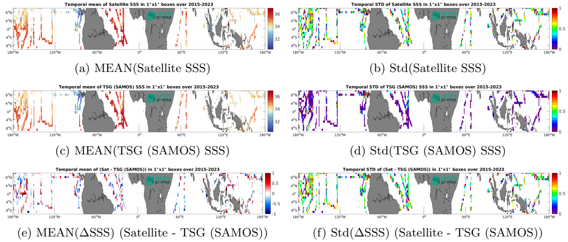
Figure 7: Temporal mean (left) and Std (right) of SSS from SMAP SSS L2 v5.3 - 40 km (RSS) (top), TSG (SAMOS) (middle), and of \Delta SSS (Satellite - TSG (SAMOS)). Only match-up pairs are used to generate these maps.
