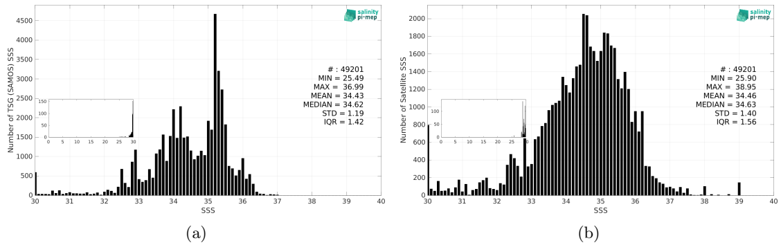
Figure 3: Histograms of SSS from TSG (SAMOS) (a) and SMAP SSS L2 v5.3 - 40 km (RSS) (b) considering all match-up pairs per bins of 0.1 over the Equatorial Ocean 10N-10S Pi-MEP region and for the full satellite product period.
