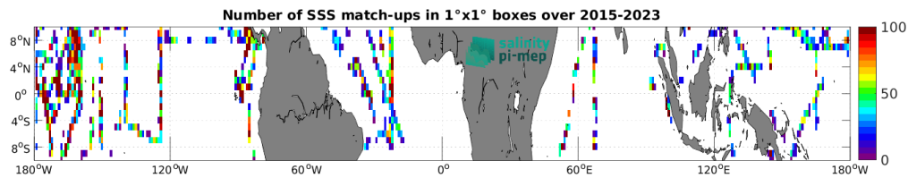
Figure 5: Number of SSS match-ups between TSG (SAMOS) SSS and the SMAP SSS L2 v5.3 - 40 km (RSS) SSS product for the Equatorial Ocean 10N-10S Pi-MEP region over 1^\circ \times 1^\circ boxes and for the full satellite product period.
