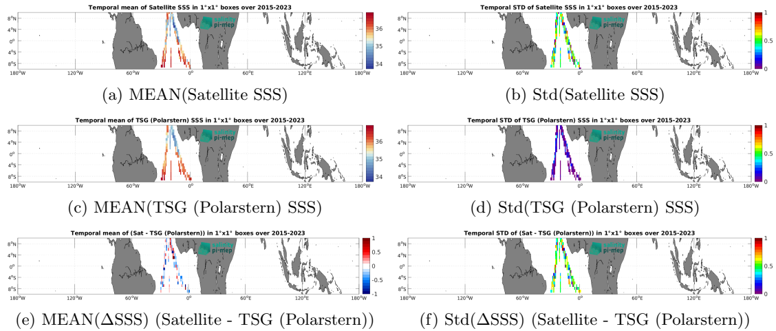
Figure 7: Temporal mean (left) and Std (right) of SSS from SMAP SSS L2 v5.3 - 40 km (RSS) (top), TSG (Polarstern) (middle), and of \Delta SSS (Satellite - TSG (Polarstern)). Only match-up pairs are used to generate these maps.
