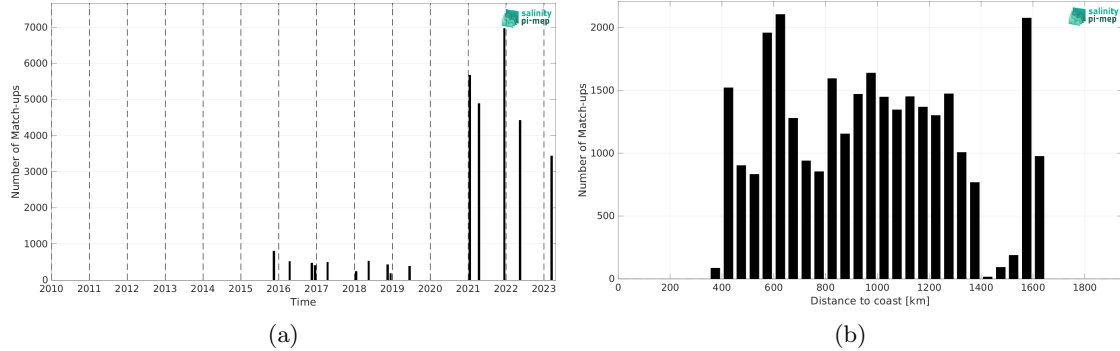
Figure 2: Number of match-ups between TSG (Polarstern) and SMAP SSS L2 v5.3 - 40 km (RSS) SSS as a function of time (a) and as function of the distance to coast (b) over the Equatorial Ocean 10N-10S Pi-MEP region and for the full satellite product period.
