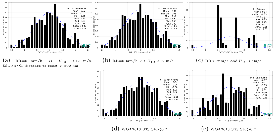
Figure 15: Normalized histogram of \Delta\text{SSS} (SMAP SSS L2 v5.3 - 40 km (RSS) - TSG (Polarstern)) for 5 different subdatasets corresponding to: RR=0 mm/h, 3 < U_{10} < 12 m/s, SST>5°C, distance to coast > 800 km (a), RR=0 mm/h, 3 < U_{10} < 12 m/s (b), RR>1mm/h and U_{10} < 4 m/s (c), WOA2013 SSS Std<0.2 (d), WOA2013 SSS Std>0.2 (e).
