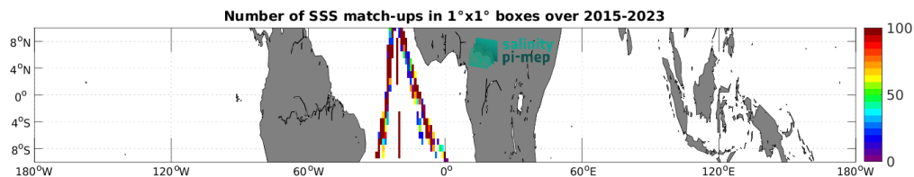
Figure 5: Number of SSS match-ups between TSG (Polarstern) SSS and the SMAP SSS L2 v5.3 - 40 km (RSS) SSS product for the Equatorial Ocean 10N-10S Pi-MEP region over 1^\circ \times 1^\circ boxes and for the full satellite product period.
