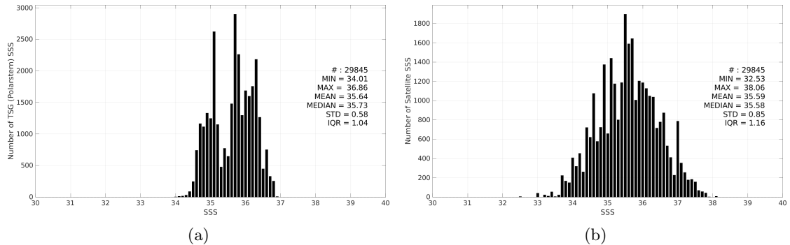
Figure 3: Histograms of SSS from TSG (Polarstern) (a) and SMAP SSS L2 v5.3 - 40 km (RSS) (b) considering all match-up pairs per bins of 0.1 over the Equatorial Ocean 10N-10S Pi-MEP region and for the full satellite product period.
