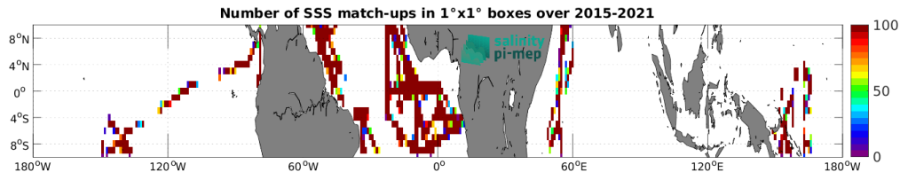
Figure 5: Number of SSS match-ups between TSG (GOSUD-Research-vessel) SSS and the SMAP SSS L2 v5.3 - 40 km (RSS) SSS product for the Equatorial Ocean 10N-10S Pi-MEP region over 1^\circ \times 1^\circ boxes and for the full satellite product period.
