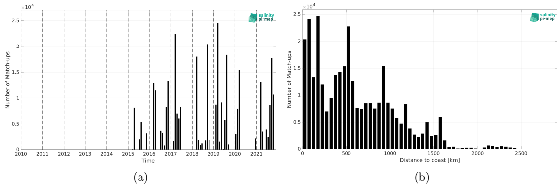
Figure 2: Number of match-ups between TSG (GOSUD-Research-vessel) and SMAP SSS L2 v5.3 - 40 km (RSS) SSS as a function of time (a) and as function of the distance to coast (b) over the Equatorial Ocean 10N-10S Pi-MEP region and for the full satellite product period.
