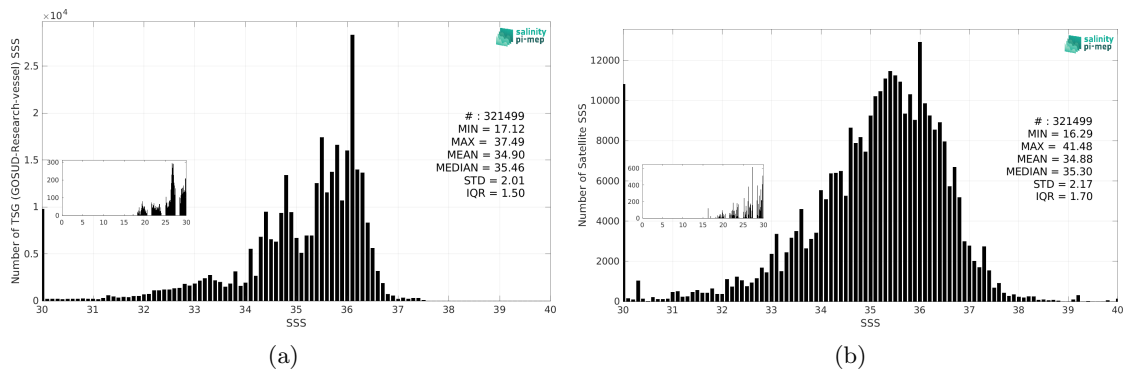
Figure 3: Histograms of SSS from TSG (GOSUD-Research-vessel) (a) and SMAP SSS L2 v5.3 - 40 km (RSS) (b) considering all match-up pairs per bins of 0.1 over the Equatorial Ocean 10N-10S Pi-MEP region and for the full satellite product period.
