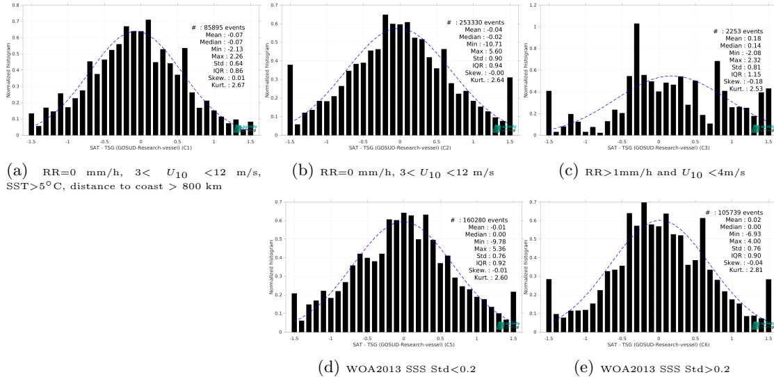
Figure 15: Normalized histogram of \Delta SSS (SMAP SSS L2 v5.3 - 40 km (RSS) - TSG (GOSUD-Research-vessel)) for 5 different subdatasets corresponding to: RR=0 mm/h, 3 < U_{10} < 12 m/s, SST >5^\circ\text{C} , distance to coast > 800 km (a), RR=0 mm/h, 3 < U_{10} < 12 m/s (b), RR >1 mm/h and U_{10} < 4 m/s (c), WOA2013 SSS Std <0.2 (d), WOA2013 SSS Std >0.2 (e).
