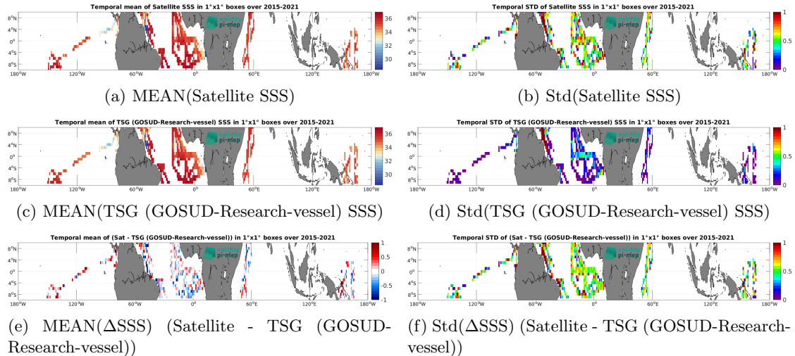
Figure 7: Temporal mean (left) and Std (right) of SSS from SMAP SSS L2 v5.3 - 40 km (RSS) (top), TSG (GOSUD-Research-vessel) (middle), and of \Delta SSS (Satellite - TSG (GOSUD-Research-vessel)). Only match-up pairs are used to generate these maps.
