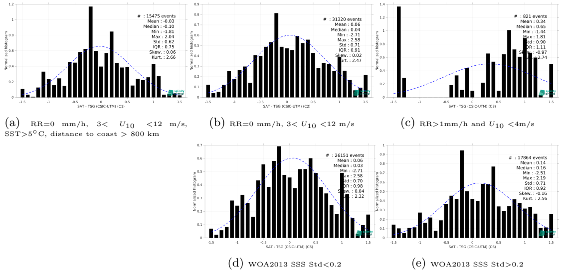
Figure 15: Normalized histogram of \Delta SSS (SMAP SSS L2 v5.3 - 40 km (RSS) - TSG (CSIC-UTM)) for 5 different subdatasets corresponding to: RR=0 mm/h, 3 < U_{10} < 12 m/s, SST>5°C, distance to coast > 800 km (a), RR=0 mm/h, 3 < U_{10} < 12 m/s (b), RR>1mm/h and U_{10} < 4 m/s (c), WOA2013 SSS Std<0.2 (d), WOA2013 SSS Std>0.2 (e).
