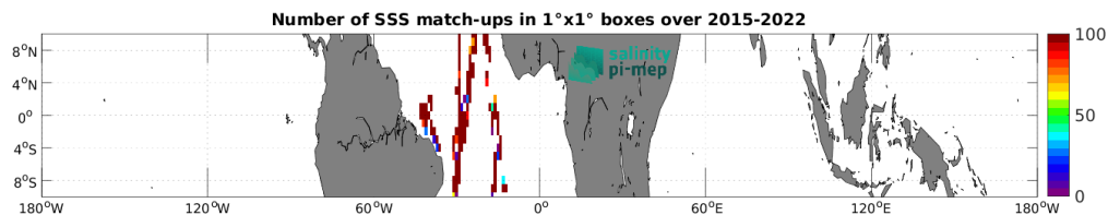
Figure 5: Number of SSS match-ups between TSG (CSIC-UTM) SSS and the SMAP SSS L2 v5.3 - 40 km (RSS) SSS product for the Equatorial Ocean 10N-10S Pi-MEP region over 1^\circ \times 1^\circ boxes and for the full satellite product period.
