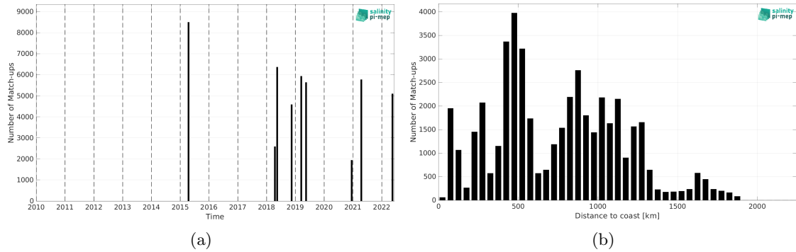
Figure 2: Number of match-ups between TSG (CSIC-UTM) and SMAP SSS L2 v5.3 - 40 km (RSS) SSS as a function of time (a) and as function of the distance to coast (b) over the Equatorial Ocean 10N-10S Pi-MEP region and for the full satellite product period.
