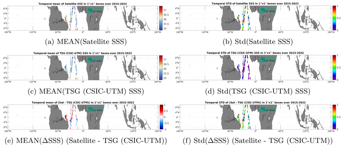
Figure 7: Temporal mean (left) and Std (right) of SSS from SMAP SSS L2 v5.3 - 40 km (RSS) (top), TSG (CSIC-UTM) (middle), and of \Delta SSS (Satellite - TSG (CSIC-UTM)). Only match-up pairs are used to generate these maps.
