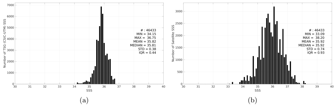
Figure 3: Histograms of SSS from TSG (CSIC-UTM) (a) and SMAP SSS L2 v5.3 - 40 km (RSS) (b) considering all match-up pairs per bins of 0.1 over the Equatorial Ocean 10N-10S Pi-MEP region and for the full satellite product period.
