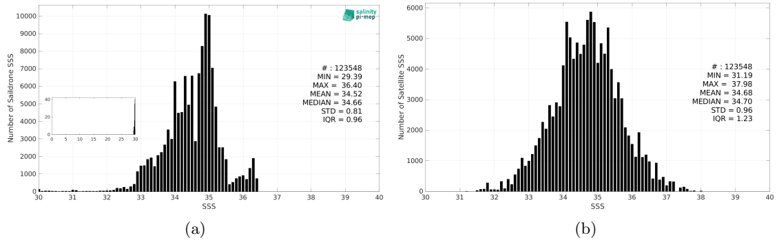
Figure 3: Histograms of SSS from Saildrone (a) and SMAP SSS L2 v5.3 - 40 km (RSS) (b) considering all match-up pairs per bins of 0.1 over the Equatorial Ocean 10N-10S Pi-MEP region and for the full satellite product period.
