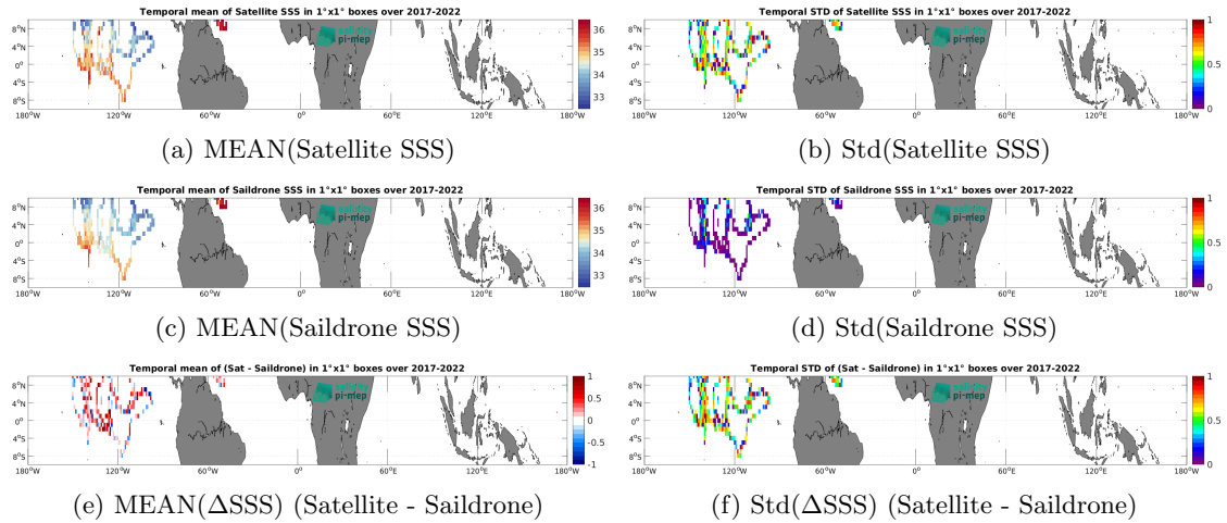
Figure 7: Temporal mean (left) and Std (right) of SSS from SMAP SSS L2 v5.3 - 40 km (RSS) (top), Saildrone (middle), and of \Delta SSS (Satellite - Saildrone). Only match-up pairs are used to generate these maps.
