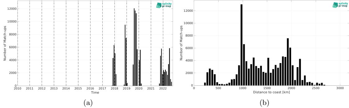
Figure 2: Number of match-ups between Saildrone and SMAP SSS L2 v5.3 - 40 km (RSS) SSS as a function of time (a) and as function of the distance to coast (b) over the Equatorial Ocean 10N-10S Pi-MEP region and for the full satellite product period.
