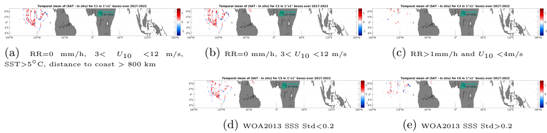
Figure 14: Temporal mean gridded over spatial boxes of size 1^\circ \times 1^\circ of \Delta SSS (SMAP SSS L2 v5.3 - 40 km (RSS) - Saildrone) for 5 different subdatasets corresponding to:RR=0 mm/h, 3 < U_{10} < 12 m/s, SST>5°C, distance to coast > 800 km (a), RR=0 mm/h, 3 < U_{10} < 12 m/s (b), RR>1mm/h and U_{10} < 4 m/s (c), WOA2013 SSS Std<0.2 (d), WOA2013 SSS Std>0.2 (e).
