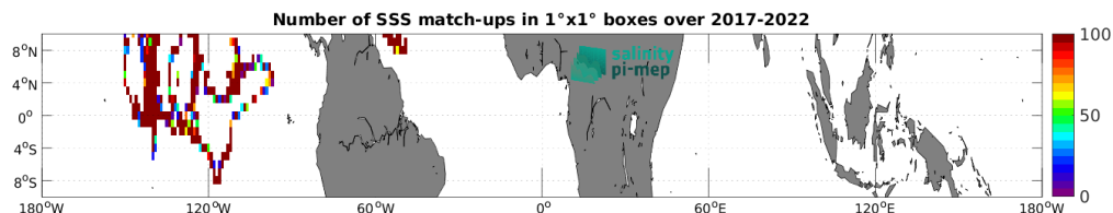
Figure 5: Number of SSS match-ups between Saildrone SSS and the SMAP SSS L2 v5.3 - 40 km (RSS) SSS product for the Equatorial Ocean 10N-10S Pi-MEP region over 1^\circ \times 1^\circ boxes and for the full satellite product period.
