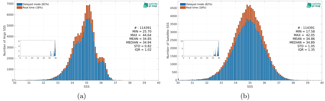
Figure 3: Histograms of SSS from Argo (a) and SMAP SSS L2 v5.3 - 40 km (RSS) (b) considering all match-up pairs per bins of 0.1 over the Equatorial Ocean 10N-10S Pi-MEP region and for the full satellite product period.
