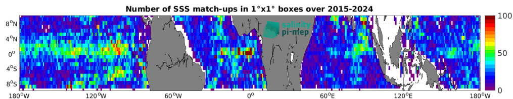
Figure 5: Number of SSS match-ups between Argo SSS and the SMAP SSS L2 v5.3 - 40 km (RSS) SSS product for the Equatorial Ocean 10N-10S Pi-MEP region over 1^\circ \times 1^\circ boxes and for the full satellite product period.
