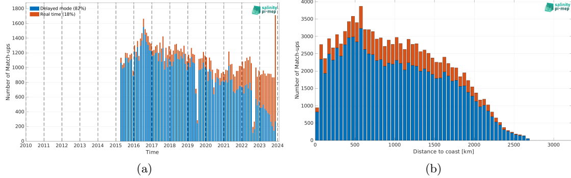
Figure 2: Number of match-ups between Argo and SMAP SSS L2 v5.3 - 40 km (RSS) SSS as a function of time (a) and as function of the distance to coast (b) over the Equatorial Ocean 10N-10S Pi-MEP region and for the full satellite product period.
