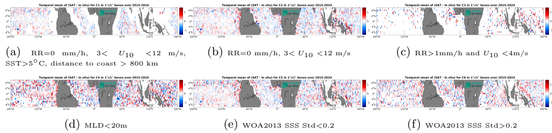
Figure 14: Temporal mean gridded over spatial boxes of size 1^\circ \times 1^\circ of \Delta\text{SSS} (SMAP SSS L2 v5.3 - 40 km (RSS) - Argo) for 6 different subdatasets corresponding to:RR=0 mm/h, 3 < U_{10} < 12 m/s, SST>5°C, distance to coast > 800 km (a), RR=0 mm/h, 3 < U_{10} < 12 m/s (b), RR>1mm/h and U_{10} < 4 m/s (c),MLD<20m (d),WOA2013 SSS Std<0.2 (e),WOA2013 SSS Std>0.2 (f).
