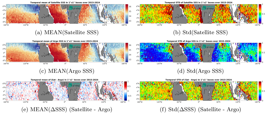
Figure 7: Temporal mean (left) and Std (right) of SSS from SMAP SSS L2 v5.3 - 40 km (RSS) (top), Argo (middle), and of \Delta SSS (Satellite - Argo). Only match-up pairs are used to generate these maps.
