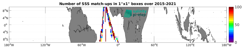
Figure 4: Number of SSS match-ups between TSG (Polarstern) SSS and the SMAP SSS L2 v5 - 40 km (RSS) SSS product for the Equatorial Ocean 10N-10S Pi-MEP region over 1^\circ \times 1^\circ boxes and for the full satellite product period.
