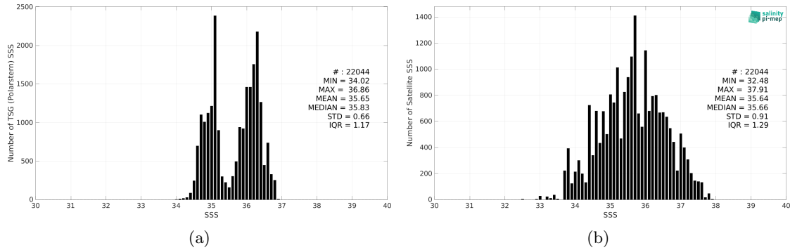
Figure 2: Histograms of SSS from TSG (Polarstern) (a) and SMAP SSS L2 v5 - 40 km (RSS) (b) considering all match-up pairs per bins of 0.1 over the Equatorial Ocean 10N-10S Pi-MEP region and for the full satellite product period.
