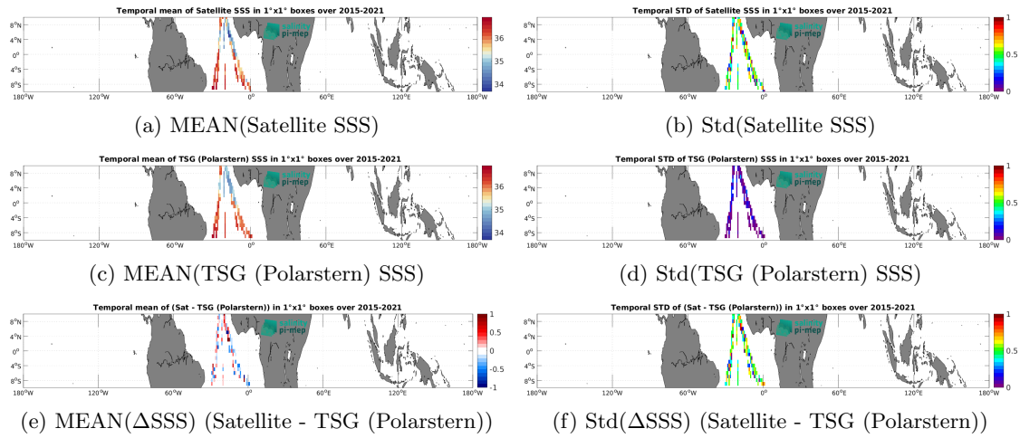
Figure 6: Temporal mean (left) and Std (right) of SSS from SMAP SSS L2 v5 - 40 km (RSS) (top), TSG (Polarstern) (middle), and of \Delta SSS (Satellite - TSG (Polarstern)). Only match-up pairs are used to generate these maps.
