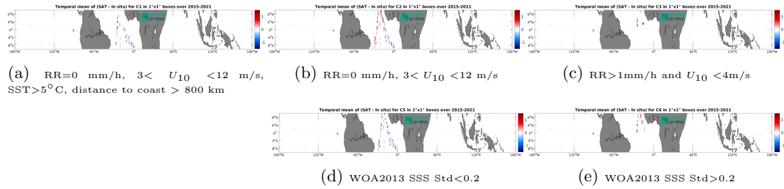
Figure 12: Temporal mean gridded over spatial boxes of size 1^\circ \times 1^\circ of \Delta SSS (SMAP SSS L2 v5 - 40 km (RSS) - TSG (Polarstern)) for 5 different subdatasets corresponding to:RR=0 mm/h, 3 < U_{10} < 12 m/s, SST >5^\circ\text{C} , distance to coast > 800 km (a), RR=0 mm/h, 3 < U_{10} < 12 m/s (b), RR >1 mm/h and U_{10} < 4 m/s (c), WOA2013 SSS Std <0.2 (d), WOA2013 SSS Std >0.2 (e).
