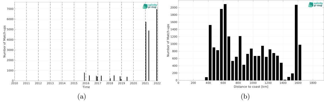
Figure 1: Number of match-ups between TSG (Polarstern) and SMAP SSS L2 v5 - 40 km (RSS) SSS as a function of time (a) and as function of the distance to coast (b) over the Equatorial Ocean 10N-10S Pi-MEP region and for the full satellite product period.
