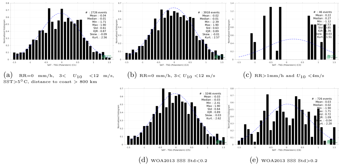
Figure 13: Normalized histogram of \Delta SSS (SMAP SSS L2 v5 - 40 km (RSS) - TSG (Polarstern)) for 5 different subdatasets corresponding to: RR=0 mm/h, 3 < U_{10} < 12 m/s, SST > 5^\circ C , distance to coast > 800 km (a), RR=0 mm/h, 3 < U_{10} < 12 m/s (b), RR > 1 mm/h and U_{10} < 4 m/s (c), WOA2013 SSS Std < 0.2 (d), WOA2013 SSS Std > 0.2 (e).
