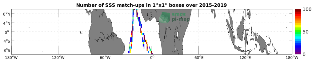
Figure 4: Number of SSS match-ups between TSG (Polarstern) SSS and the SMAP SSS L2 v5 - 40 km (RSS) SSS product for the Equatorial Ocean 10N-10S Pi-MEP region over 1^\circ \times 1^\circ boxes and for the full satellite product period.
