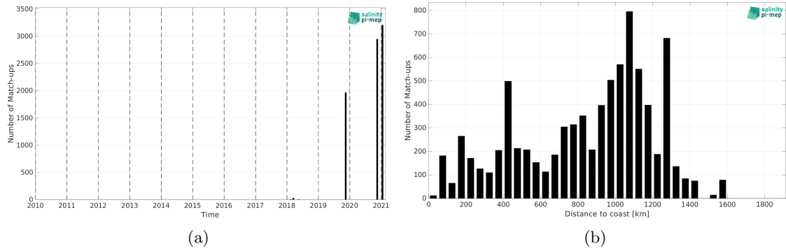
Figure 1: Number of match-ups between TSG (GOSUD-Sailing-ship) and SMAP SSS L2 v5 - 40 km (RSS) SSS as a function of time (a) and as function of the distance to coast (b) over the Equatorial Ocean 10N-10S Pi-MEP region and for the full satellite product period.
