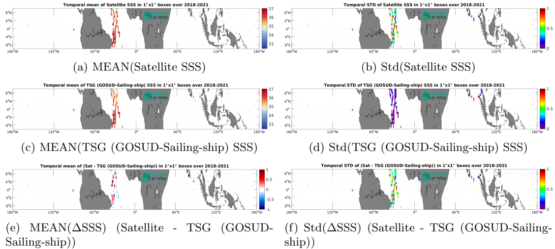
Figure 6: Temporal mean (left) and Std (right) of SSS from SMAP SSS L2 v5 - 40 km (RSS) (top), TSG (GOSUD-Sailing-ship) (middle), and of \Delta SSS (Satellite - TSG (GOSUD-Sailing-ship)). Only match-up pairs are used to generate these maps.
