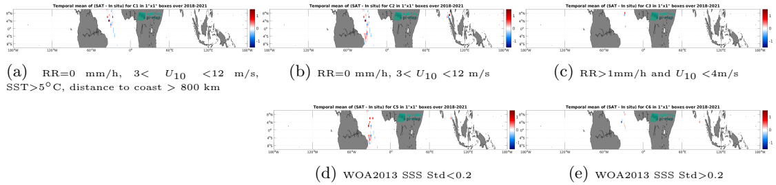
Figure 12: Temporal mean gridded over spatial boxes of size 1^\circ \times 1^\circ of \Delta SSS (SMAP SSS L2 v5 - 40 km (RSS) - TSG (GOSUD-Sailing-ship)) for 5 different subdatasets corresponding to:RR=0 mm/h, 3 < U_{10} < 12 m/s, SST>5°C, distance to coast > 800 km (a), RR=0 mm/h, 3 < U_{10} < 12 m/s (b), RR>1mm/h and U_{10} < 4 m/s (c), WOA2013 SSS Std<0.2 (d), WOA2013 SSS Std>0.2 (e).
