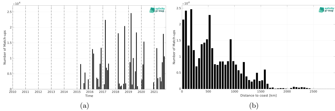
Figure 1: Number of match-ups between TSG (GOSUD-Research-vessel) and SMAP SSS L2 v5 - 40 km (RSS) SSS as a function of time (a) and as function of the distance to coast (b) over the Equatorial Ocean 10N-10S Pi-MEP region and for the full satellite product period.
