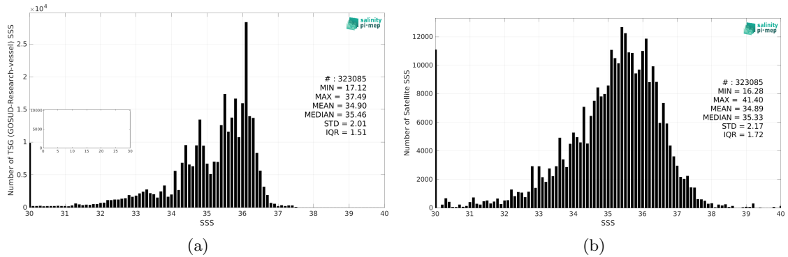
Figure 2: Histograms of SSS from TSG (GOSUD-Research-vessel) (a) and SMAP SSS L2 v5 - 40 km (RSS) (b) considering all match-up pairs per bins of 0.1 over the Equatorial Ocean 10N-10S Pi-MEP region and for the full satellite product period.
