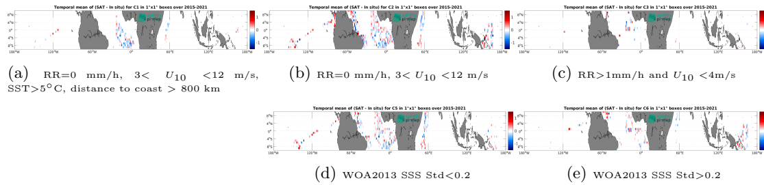
Figure 12: Temporal mean gridded over spatial boxes of size 1^\circ \times 1^\circ of \Delta\text{SSS} (SMAP SSS L2 v5 - 40 km (RSS) - TSG (GOSUD-Research-vessel)) for 5 different subdatasets corresponding to: RR=0 mm/h, 3 < U_{10} < 12 m/s, SST>5°C, distance to coast > 800 km (a), RR=0 mm/h, 3 < U_{10} < 12 m/s (b), RR>1mm/h and U_{10} < 4 m/s (c), WOA2013 SSS Std<0.2 (d), WOA2013 SSS Std>0.2 (e).
