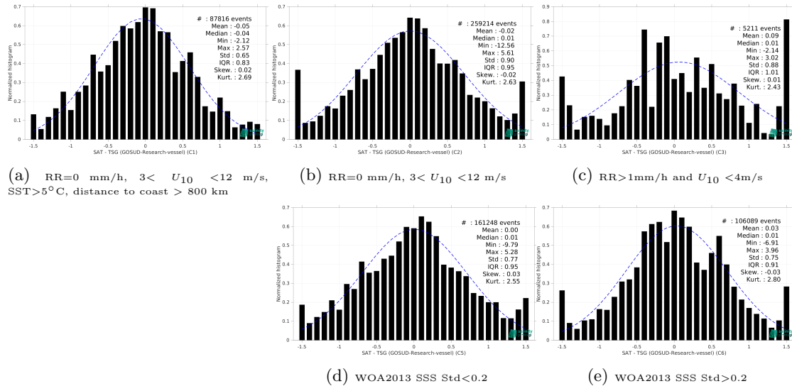
Figure 13: Normalized histogram of \Delta\text{SSS} (SMAP SSS L2 v5 - 40 km (RSS) - TSG (GOSUD-Research-vessel)) for 5 different subdatasets corresponding to: RR=0 mm/h, 3 < U_{10} < 12 m/s, SST>5°C, distance to coast > 800 km (a), RR=0 mm/h, 3 < U_{10} < 12 m/s (b), RR>1mm/h and U_{10} < 4 m/s (c), WOA2013 SSS Std<0.2 (d), WOA2013 SSS Std>0.2 (e).
