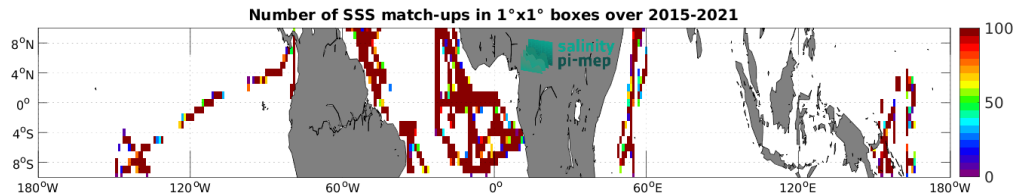
Figure 4: Number of SSS match-ups between TSG (GOSUD-Research-vessel) SSS and the SMAP SSS L2 v5 - 40 km (RSS) SSS product for the Equatorial Ocean 10N-10S Pi-MEP region over 1^\circ \times 1^\circ boxes and for the full satellite product period.
