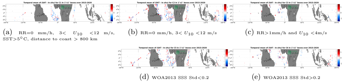
Figure 12: Temporal mean gridded over spatial boxes of size 1^\circ \times 1^\circ of \Delta SSS (SMAP SSS L2 v5 - 40 km (RSS) - TSG (GOSUD-Research-vessel)) for 5 different subdatasets corresponding to: RR=0 mm/h, 3 < U_{10} < 12 m/s, SST>5°C, distance to coast > 800 km (a), RR=0 mm/h, 3 < U_{10} < 12 m/s (b), RR>1mm/h and U_{10} < 4 m/s (c), WOA2013 SSS Std<0.2 (d), WOA2013 SSS Std>0.2 (e).
