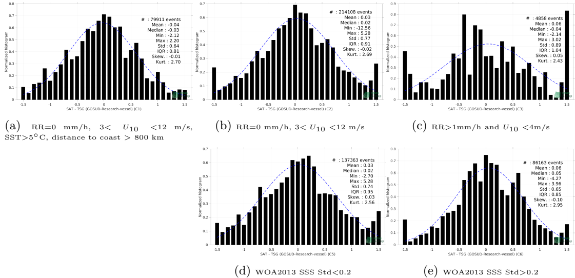
Figure 13: Normalized histogram of \Delta SSS (SMAP SSS L2 v5 - 40 km (RSS) - TSG (GOSUD-Research-vessel)) for 5 different subdatasets corresponding to: RR=0 mm/h, 3 < U_{10} < 12 m/s, SST>5°C, distance to coast > 800 km (a), RR=0 mm/h, 3 < U_{10} < 12 m/s (b), RR>1mm/h and U_{10} < 4 m/s (c), WOA2013 SSS Std<0.2 (d), WOA2013 SSS Std>0.2 (e).
