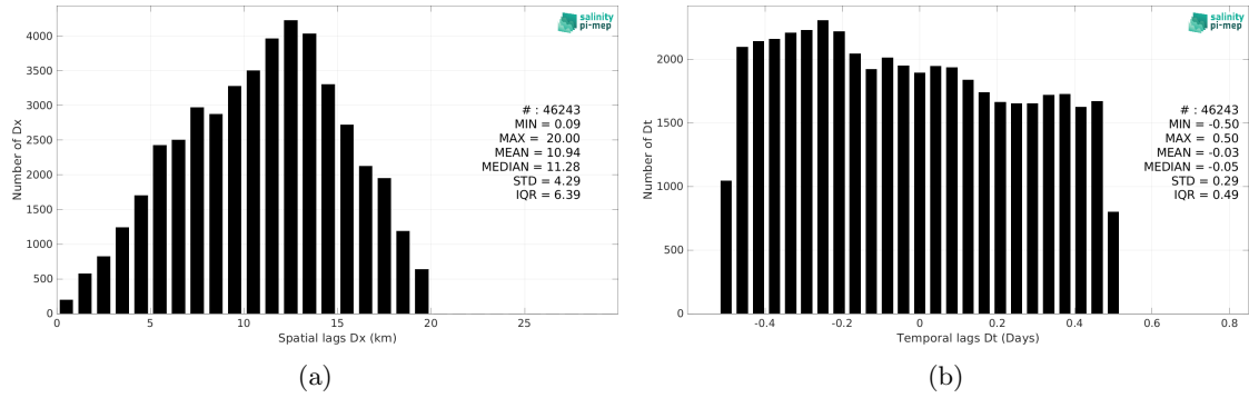
Figure 5: Histograms of the spatial (a) and temporal (b) lags between the location/time of the TSG (CSIC-UTM) measurement and the date of the corresponding SMAP SSS L2 v5 - 40 km (RSS) SSS pixel.
