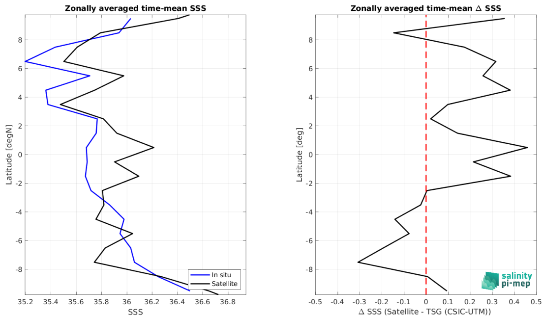
Figure 8: Left panel: Zonal mean SSS from SMAP SSS L2 v5 - 40 km (RSS) satellite product (black) and from TSG (CSIC-UTM) (blue). Right panel: Zonal mean of \Delta SSS (Satellite - TSG (CSIC-UTM)) for all the collected Pi-MEP match-up pairs estimated over the full satellite product period.
