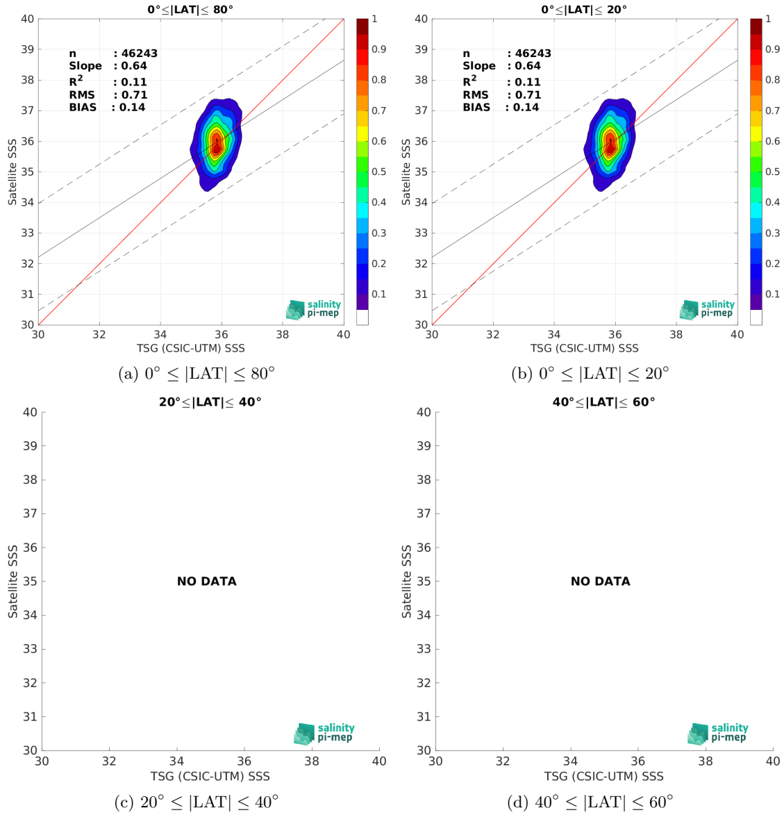
Figure 9: Contour maps of the concentration of SMAP SSS L2 v5 - 40 km (RSS) SSS (y-axis) versus TSG (CSIC-UTM) SSS (x-axis) at match-up pairs for different latitude bands. For each plot, the red line shows x=y . The black thin and dashed lines indicate a linear fit through the data cloud and the \pm 95\% confidence levels, respectively. The number match-up pairs n , the slope and R^2 coefficient of the linear fit, the root mean square (RMS) and the mean bias between satellite and in situ data are indicated for each latitude band in each plots.
