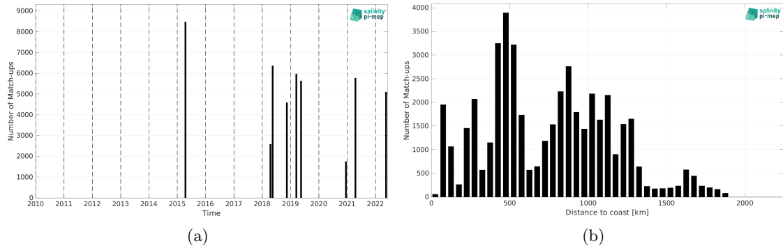
Figure 1: Number of match-ups between TSG (CSIC-UTM) and SMAP SSS L2 v5 - 40 km (RSS) SSS as a function of time (a) and as function of the distance to coast (b) over the Equatorial Ocean 10N-10S Pi-MEP region and for the full satellite product period.
