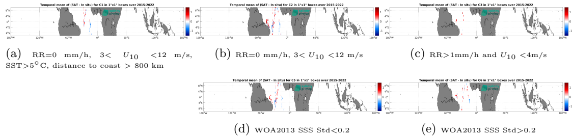
Figure 12: Temporal mean gridded over spatial boxes of size 1^\circ \times 1^\circ of \Delta SSS (SMAP SSS L2 v5 - 40 km (RSS) - TSG (CSIC-UTM)) for 5 different subdatasets corresponding to: RR=0 mm/h, 3 < U_{10} < 12 m/s, SST >5^\circ\text{C} , distance to coast > 800 km (a), RR=0 mm/h, 3 < U_{10} < 12 m/s (b), RR >1 mm/h and U_{10} < 4 m/s (c), WOA2013 SSS Std <0.2 (d), WOA2013 SSS Std >0.2 (e).
