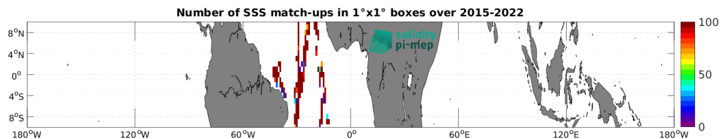
Figure 4: Number of SSS match-ups between TSG (CSIC-UTM) SSS and the SMAP SSS L2 v5 - 40 km (RSS) SSS product for the Equatorial Ocean 10N-10S Pi-MEP region over 1^\circ \times 1^\circ boxes and for the full satellite product period.
