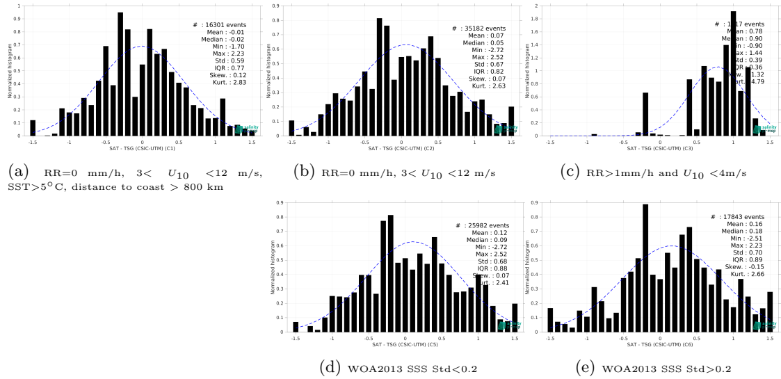
Figure 13: Normalized histogram of \Delta SSS (SMAP SSS L2 v5 - 40 km (RSS) - TSG (CSIC-UTM)) for 5 different subdatasets corresponding to: RR=0 mm/h, 3 < U_{10} < 12 m/s, SST >5^\circ\text{C} , distance to coast > 800 km (a), RR=0 mm/h, 3 < U_{10} < 12 m/s (b), RR >1 mm/h and U_{10} < 4 m/s (c), WOA2013 SSS Std <0.2 (d), WOA2013 SSS Std >0.2 (e).
