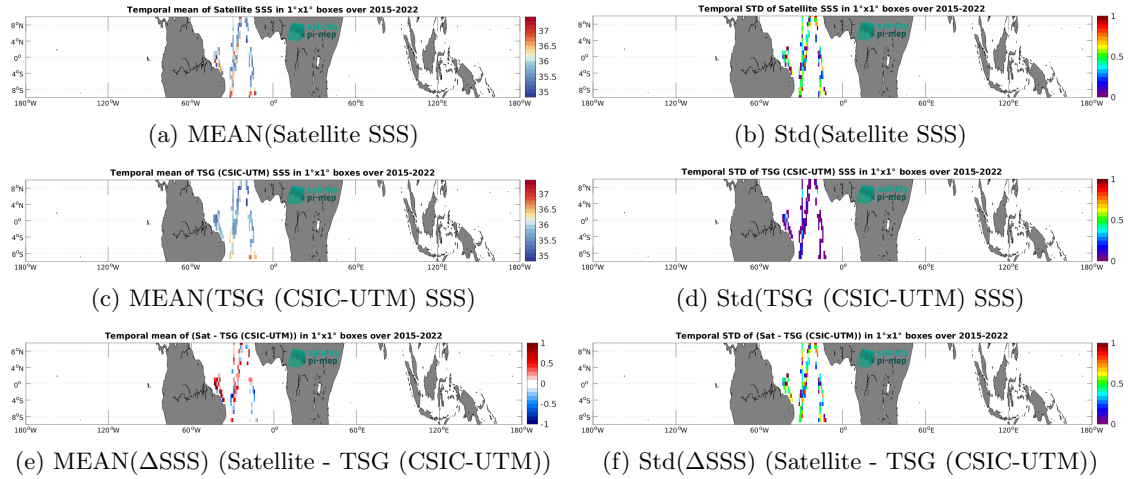
Figure 6: Temporal mean (left) and Std (right) of SSS from SMAP SSS L2 v5 - 40 km (RSS) (top), TSG (CSIC-UTM) (middle), and of \Delta SSS (Satellite - TSG (CSIC-UTM)). Only match-up pairs are used to generate these maps.
