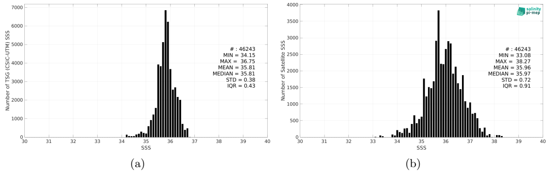
Figure 2: Histograms of SSS from TSG (CSIC-UTM) (a) and SMAP SSS L2 v5 - 40 km (RSS) (b) considering all match-up pairs per bins of 0.1 over the Equatorial Ocean 10N-10S Pi-MEP region and for the full satellite product period.
