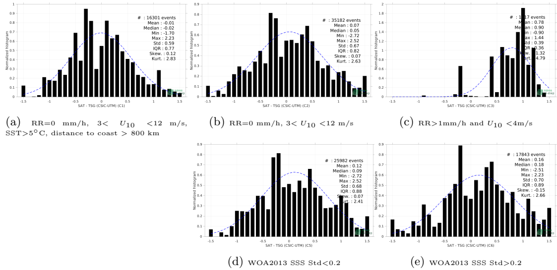
Figure 13: Normalized histogram of \Delta SSS (SMAP SSS L2 v5 - 40 km (RSS) - TSG (CSIC-UTM)) for 5 different subdatasets corresponding to: RR=0 mm/h, 3 < U_{10} < 12 m/s, SST > 5^\circ\text{C} , distance to coast > 800 km (a), RR=0 mm/h, 3 < U_{10} < 12 m/s (b), RR > 1mm/h and U_{10} < 4 m/s (c), WOA2013 SSS Std < 0.2 (d), WOA2013 SSS Std > 0.2 (e).
