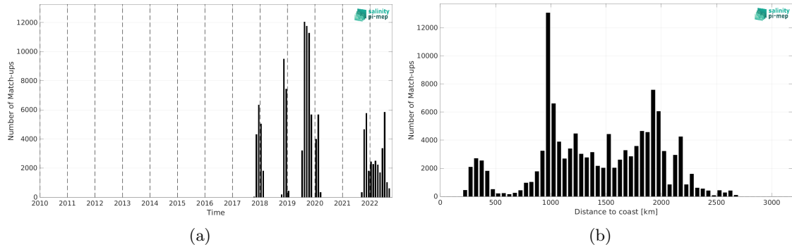
Figure 1: Number of match-ups between Sairdrone and SMAP SSS L2 v5 - 40 km (RSS) SSS as a function of time (a) and as function of the distance to coast (b) over the Equatorial Ocean 10N-10S Pi-MEP region and for the full satellite product period.
