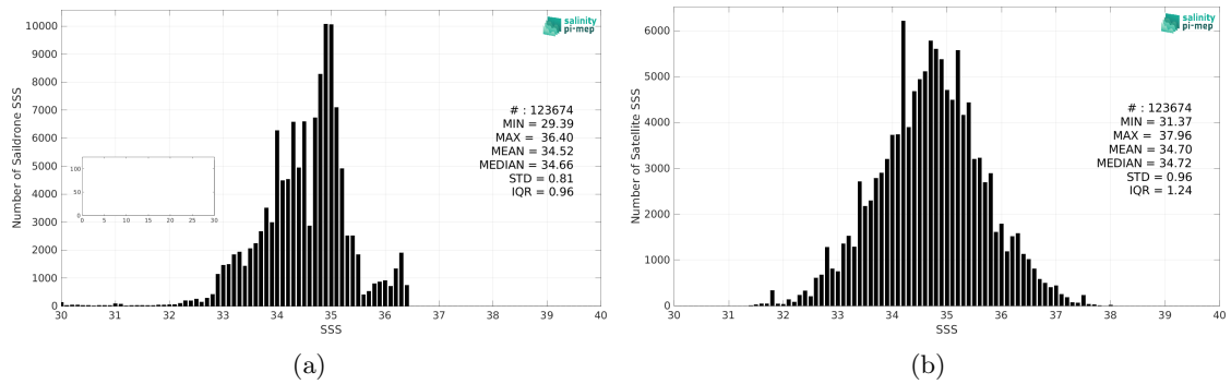
Figure 2: Histograms of SSS from Sairdrone (a) and SMAP SSS L2 v5 - 40 km (RSS) (b) considering all match-up pairs per bins of 0.1 over the Equatorial Ocean 10N-10S Pi-MEP region and for the full satellite product period.
