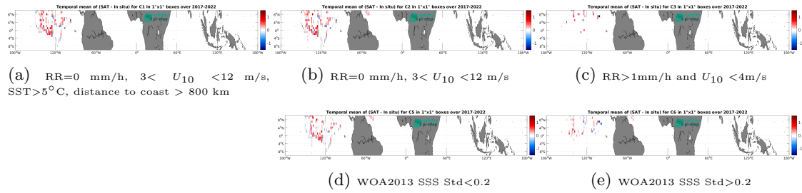
Figure 12: Temporal mean gridded over spatial boxes of size 1^\circ \times 1^\circ of \Delta SSS (SMAP SSS L2 v5 - 40 km (RSS) - Saildrone) for 5 different subdatasets corresponding to:RR=0 mm/h, 3 < U_{10} < 12 m/s, SST >5^\circ\text{C} , distance to coast > 800 km (a), RR=0 mm/h, 3 < U_{10} < 12 m/s (b), RR >1 mm/h and U_{10} < 4 m/s (c), WOA2013 SSS Std <0.2 (d), WOA2013 SSS Std >0.2 (e).
