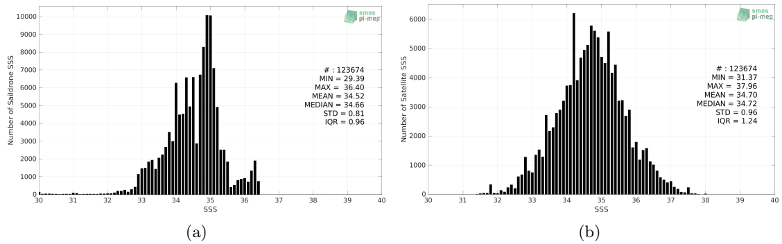
Figure 2: Histograms of SSS from Saildrone (a) and SMAP SSS L2 v5 - 40 km (RSS) (b) considering all match-up pairs per bins of 0.1 over the Equatorial Ocean 10N-10S Pi-MEP region and for the full satellite product period.
