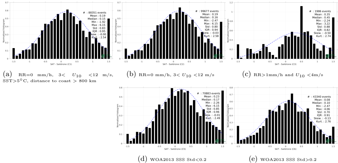
Figure 13: Normalized histogram of \Delta SSS (SMAP SSS L2 v5 - 40 km (RSS) - Saildrone) for 5 different subdatasets corresponding to: RR=0 mm/h, 3 < U_{10} < 12 m/s, SST >5^\circ\text{C} , distance to coast > 800 km (a), RR=0 mm/h, 3 < U_{10} < 12 m/s (b), RR >1 mm/h and U_{10} < 4 m/s (c), WOA2013 SSS Std <0.2 (d), WOA2013 SSS Std >0.2 (e).
