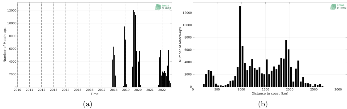
Figure 1: Number of match-ups between Saildrone and SMAP SSS L2 v5 - 40 km (RSS) SSS as a function of time (a) and as function of the distance to coast (b) over the Equatorial Ocean 10N-10S Pi-MEP region and for the full satellite product period.
