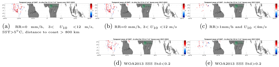
Figure 12: Temporal mean gridded over spatial boxes of size 1^\circ \times 1^\circ of \Delta SSS (SMAP SSS L2 v5 - 40 km (RSS) - Saildrone) for 5 different subdatasets corresponding to:RR=0 mm/h, 3 < U_{10} < 12 m/s, SST >5^\circ\text{C} , distance to coast > 800 km (a), RR=0 mm/h, 3 < U_{10} < 12 m/s (b), RR >1 mm/h and U_{10} < 4 m/s (c), WOA2013 SSS Std <0.2 (d), WOA2013 SSS Std >0.2 (e).
