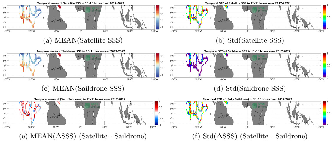
Figure 6: Temporal mean (left) and Std (right) of SSS from SMAP SSS L2 v5 - 40 km (RSS) (top), Saildrone (middle), and of \Delta SSS (Satellite - Saildrone). Only match-up pairs are used to generate these maps.
