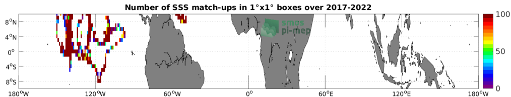
Figure 4: Number of SSS match-ups between Saildrone SSS and the SMAP SSS L2 v5 - 40 km (RSS) SSS product for the Equatorial Ocean 10N-10S Pi-MEP region over 1^\circ \times 1^\circ boxes and for the full satellite product period.
