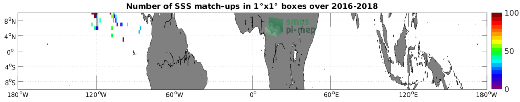
Figure 3: Number of SSS match-ups between Surface drifters SSS and the SMAP SSS L2 v5 - 40 km (RSS) SSS product for the Equatorial Ocean 10N-10S Pi-MEP region over 1^\circ \times 1^\circ boxes and for the full satellite product period.
