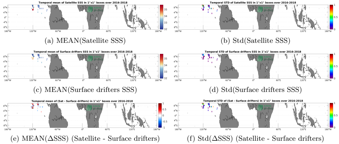
Figure 5: Temporal mean (left) and Std (right) of SSS from SMAP SSS L2 v5 - 40 km (RSS) (top), Surface drifters (middle), and of \Delta SSS (Satellite - Surface drifters). Only match-up pairs are used to generate these maps.
