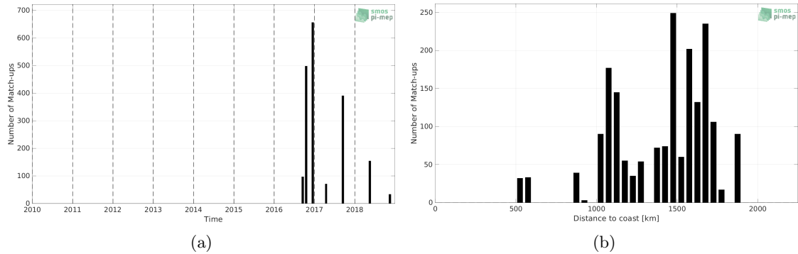
Figure 1: Number of match-ups between Surface drifters and SMAP SSS L2 v5 - 40 km (RSS) SSS as a function of time (a) and as function of the distance to coast (b) over the Equatorial Ocean 10N-10S Pi-MEP region and for the full satellite product period.
