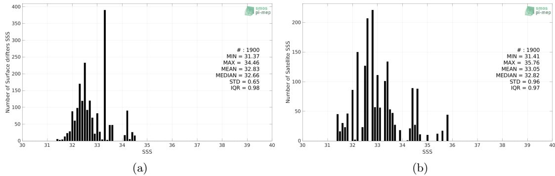
Figure 2: Histograms of SSS from Surface drifters (a) and SMAP SSS L2 v5 - 40 km (RSS) (b) considering all match-up pairs per bins of 0.1 over the Equatorial Ocean 10N-10S Pi-MEP region and for the full satellite product period.
