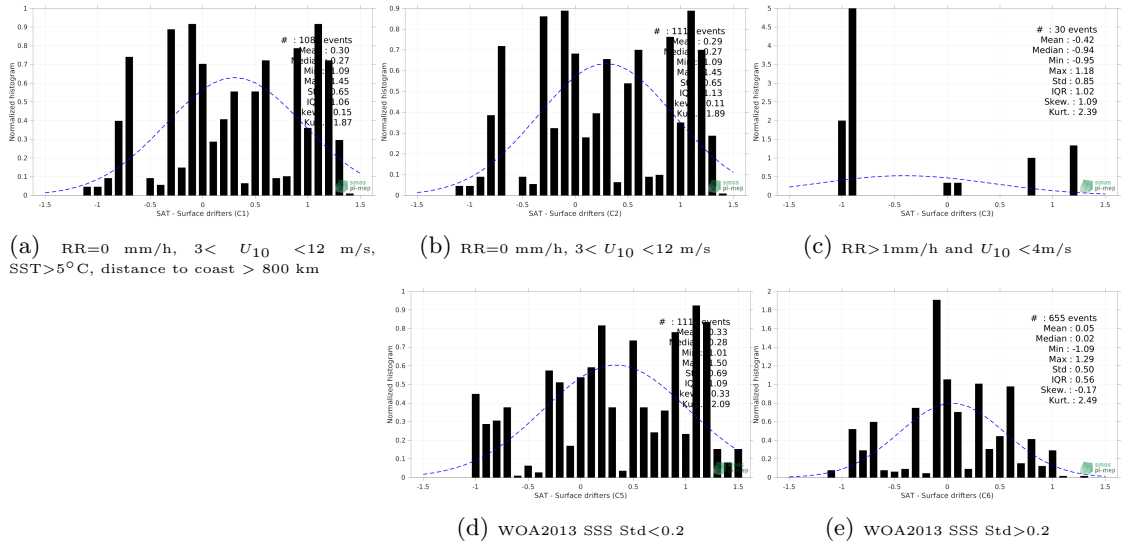
Figure 12: Normalized histogram of \Delta SSS (SMAP SSS L2 v5 - 40 km (RSS) - Surface drifters) for 5 different subdatasets corresponding to: RR=0 mm/h, 3 < U_{10} < 12 m/s, SST >5^\circ\text{C} , distance to coast > 800 km (a), RR=0 mm/h, 3 < U_{10} < 12 m/s (b), RR >1 mm/h and U_{10} < 4 m/s (c), WOA2013 SSS Std <0.2 (d), WOA2013 SSS Std >0.2 (e).
