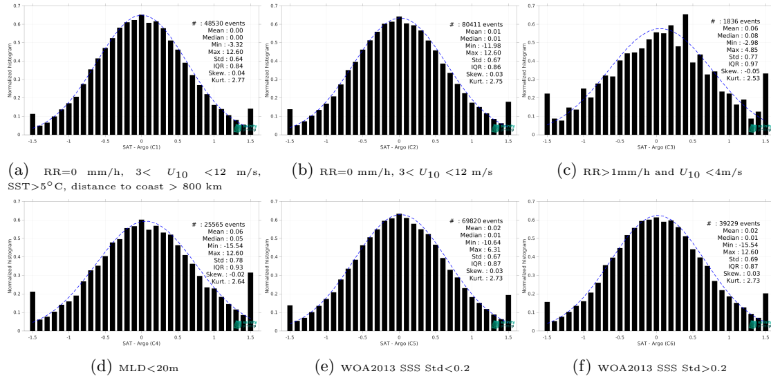
Figure 13: Normalized histogram of \Delta SSS (SMAP SSS L2 v5 - 40 km (RSS) - Argo) for 6 different subdatasets corresponding to: RR=0 mm/h, 3 < U_{10} < 12 m/s, SST >5^\circ C, distance to coast > 800 km (a), RR=0 mm/h, 3 < U_{10} < 12 m/s (b), RR >1 mm/h and U_{10} < 4 m/s (c), MLD <20 m (d), WOA2013 SSS Std <0.2 (e), WOA2013 SSS Std >0.2 (f).
