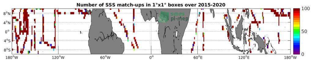
Figure 4: Number of SSS match-ups between TSG (SAMOS) SSS and the SMAP SSS L2 v4 (RSS) SSS product for the Equatorial Ocean 10N-10S Pi-MEP region over 1°x1° boxes and for the full satellite product period.
