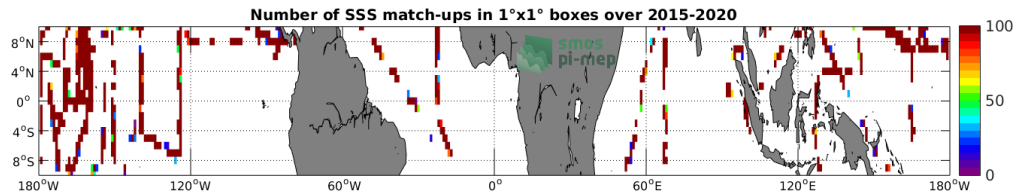
Figure 4: Number of SSS match-ups between TSG-SAMOS SSS and the SMAP-L2-RSS-V4 SSS product for the Equatorial Ocean 10N-10S Pi-MEP region over 1°x1° boxes and for the full satellite product period.
