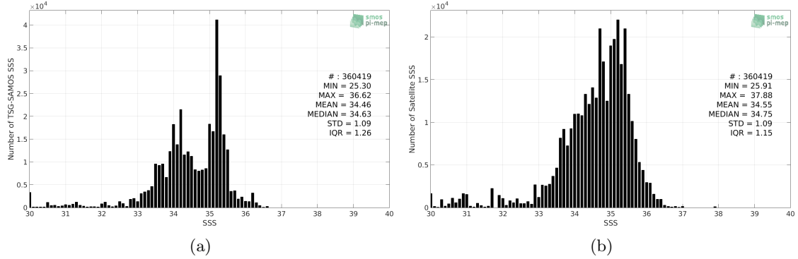
Figure 2: Histograms of SSS from TSG-SAMOS (a) and SMAP-L2-RSS-V4 (b) considering all match-up pairs per bins of 0.1 over the Equatorial Ocean 10N-10S Pi-MEP region and for the full satellite product period.
