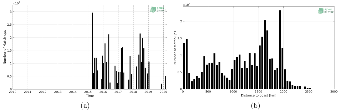
Figure 1: Number of match-ups between TSG-SAMOS and SMAP-L2-RSS-V4 SSS as a function of time (a) and as function of the distance to coast (b) over the Equatorial Ocean 10N-10S Pi-MEP region and for the full satellite product period.
