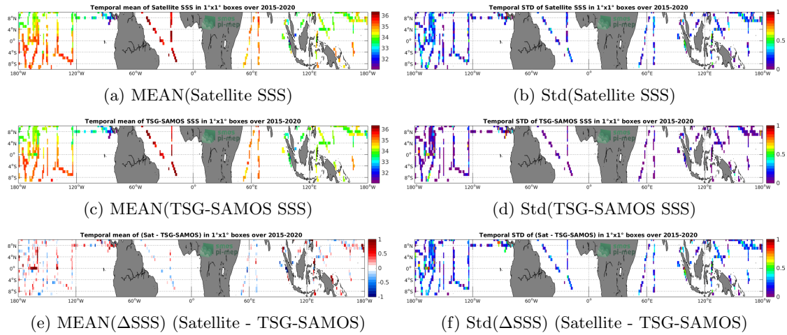
Figure 6: Temporal mean (left) and Std (right) of SSS from SMAP-L2-RSS-V4 (top), TSG-SAMOS (middle), and of \Delta SSS (Satellite - TSG-SAMOS). Only match-up pairs are used to generate these maps.
