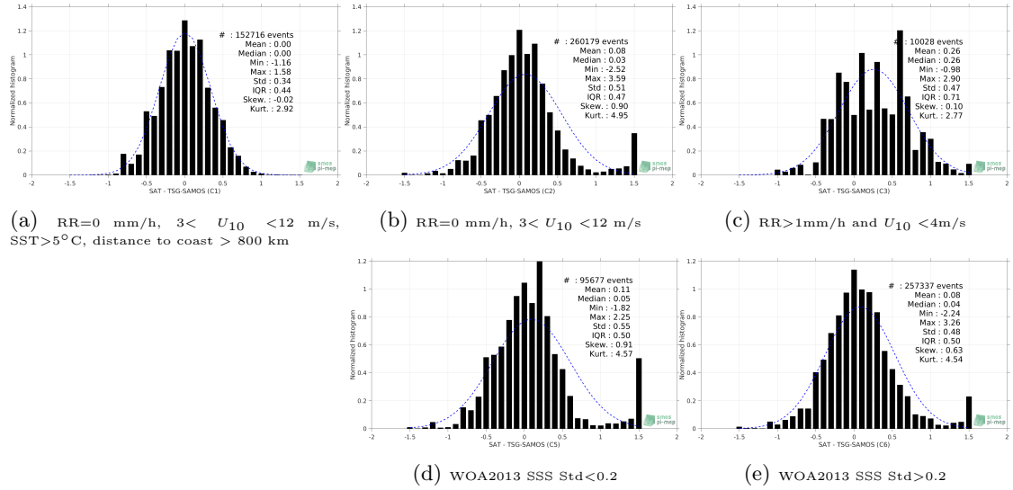
Figure 13: Normalized histogram of \Delta SSS (SMAP-L2-RSS-V4 - TSG-SAMOS) for 5 different subdatasets corresponding to: RR=0 mm/h, 3 < U_{10} < 12 m/s, SST > 5^\circ C , distance to coast > 800 km (a), RR=0 mm/h, 3 < U_{10} < 12 m/s (b), RR > 1 mm/h and U_{10} < 4 m/s (c), WOA2013 SSS Std < 0.2 (d), WOA2013 SSS Std > 0.2 (e).
