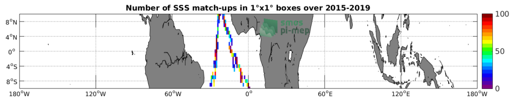
Figure 4: Number of SSS match-ups between TSG (Polarstern) SSS and the SMAP SSS L2 v4 (RSS) SSS product for the Equatorial Ocean 10N-10S Pi-MEP region over 1^\circ \times 1^\circ boxes and for the full satellite product period.
