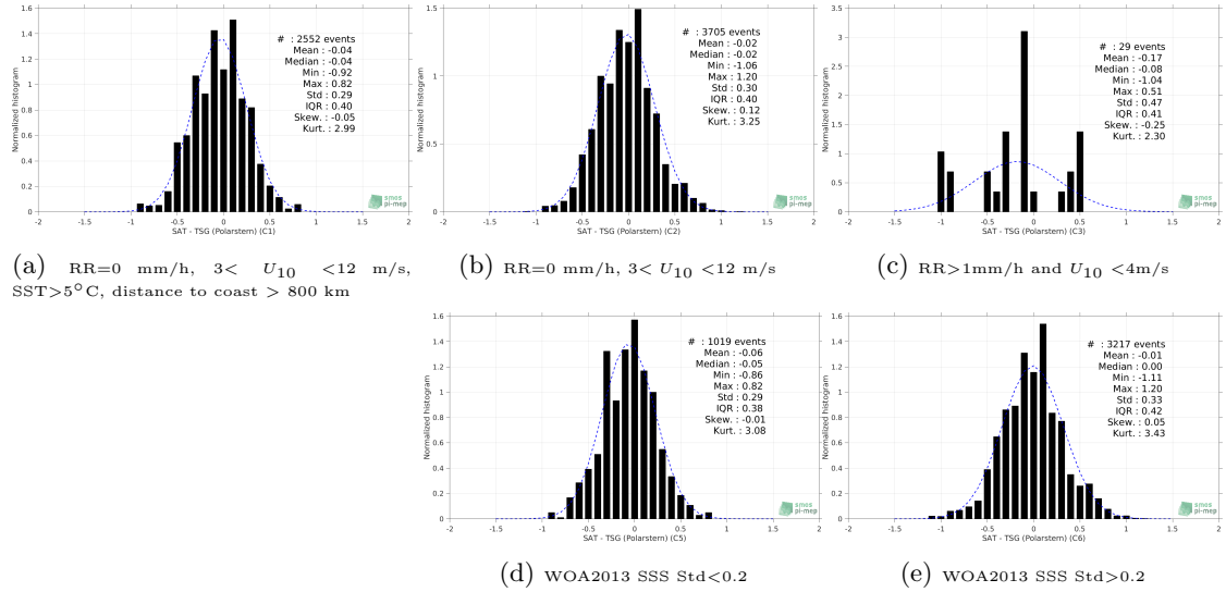
Figure 13: Normalized histogram of \Delta SSS (SMAP SSS L2 v4 (RSS) - TSG (Polarstern)) for 5 different subdatasets corresponding to: RR=0 mm/h, 3 < U_{10} < 12 m/s, SST >5^\circ\text{C} , distance to coast > 800 km (a), RR=0 mm/h, 3 < U_{10} < 12 m/s (b), RR >1 mm/h and U_{10} < 4 m/s (c), WOA2013 SSS Std <0.2 (d), WOA2013 SSS Std >0.2 (e).
