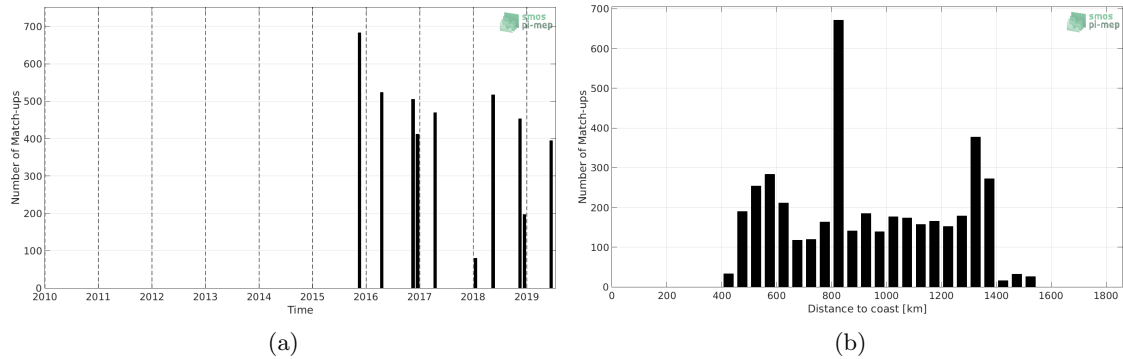
Figure 1: Number of match-ups between TSG-POLARSTERN and SMAP-L2-RSS-V4 SSS as a function of time (a) and as function of the distance to coast (b) over the Equatorial Ocean 10N-10S Pi-MEP region and for the full satellite product period.
