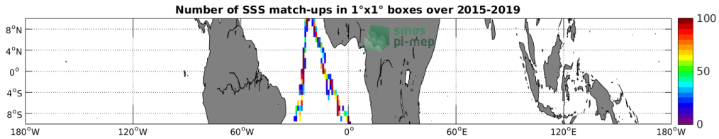
Figure 4: Number of SSS match-ups between TSG-POLARSTERN SSS and the SMAP-L2-RSS-V4 SSS product for the Equatorial Ocean 10N-10S Pi-MEP region over 1°x1° boxes and for the full satellite product period.
