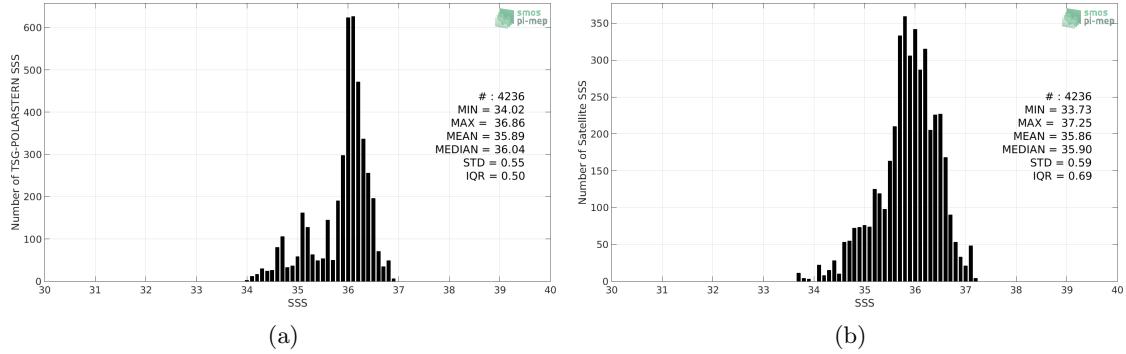
Figure 2: Histograms of SSS from TSG-POLARSTERN (a) and SMAP-L2-RSS-V4 (b) considering all match-up pairs per bins of 0.1 over the Equatorial Ocean 10N-10S Pi-MEP region and for the full satellite product period.
