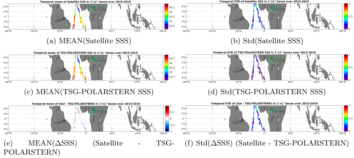
Figure 6: Temporal mean (left) and Std (right) of SSS from SMAP-L2-RSS-V4 (top), TSG-POLARSTERN (middle), and of \Delta SSS (Satellite - TSG-POLARSTERN). Only match-up pairs are used to generate these maps.
