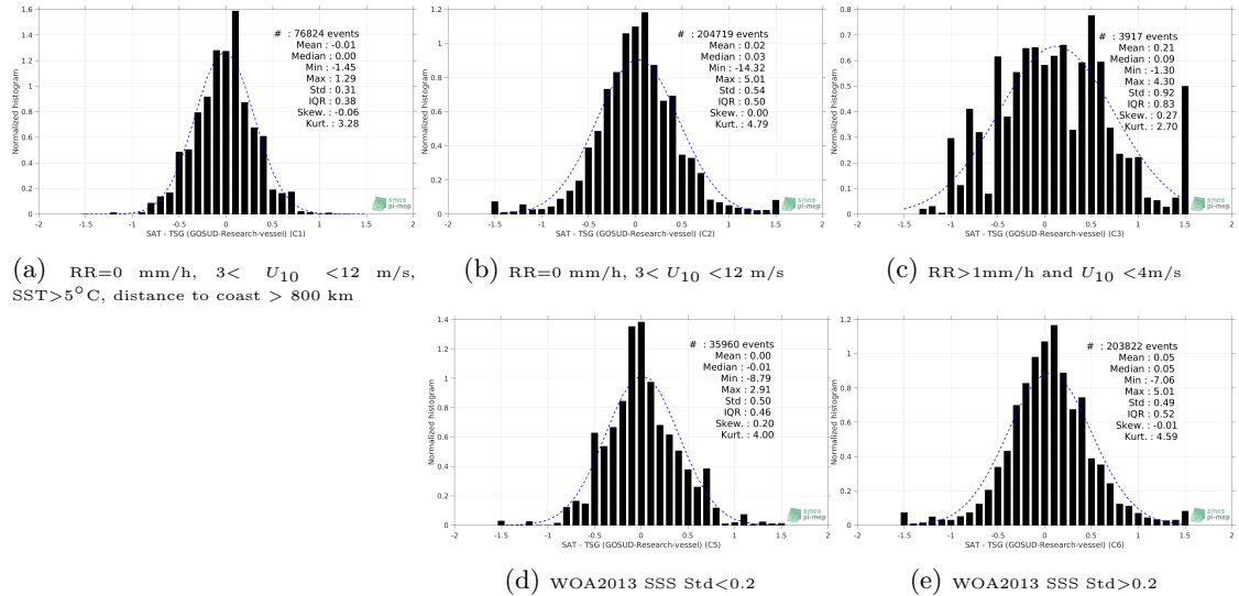
Figure 13: Normalized histogram of \Delta SSS (SMAP SSS L2 v4 (RSS) - TSG (GOSUD-Research-vessel)) for 5 different subdatasets corresponding to: RR=0 mm/h, 3 < U_{10} < 12 m/s, SST >5^\circ C, distance to coast > 800 km (a), RR=0 mm/h, 3 < U_{10} < 12 m/s (b), RR>1 mm/h and U_{10} < 4 m/s (c), WOA2013 SSS Std <0.2 (d), WOA2013 SSS Std >0.2 (e).
