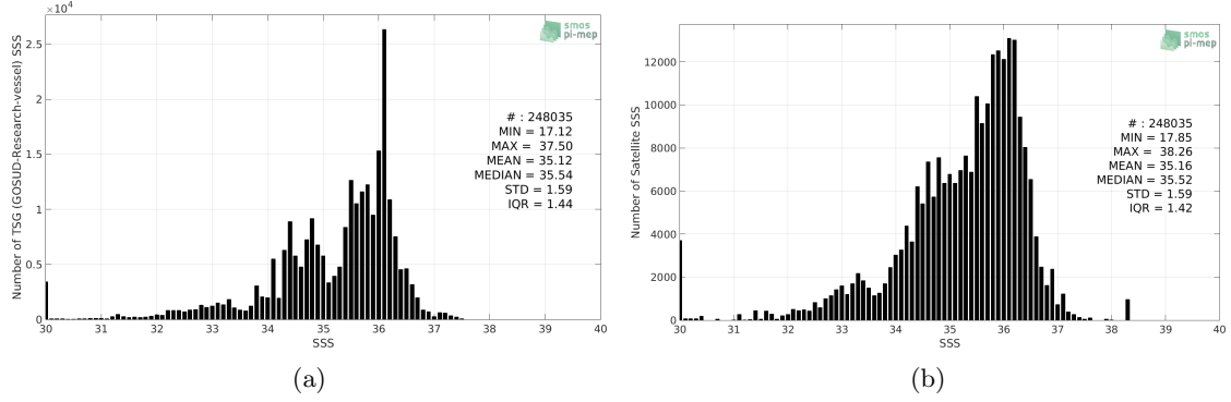
Figure 2: Histograms of SSS from TSG (GOSUD-Research-vessel) (a) and SMAP SSS L2 v4 (RSS) (b) considering all match-up pairs per bins of 0.1 over the Equatorial Ocean 10N-10S Pi-MEP region and for the full satellite product period.
