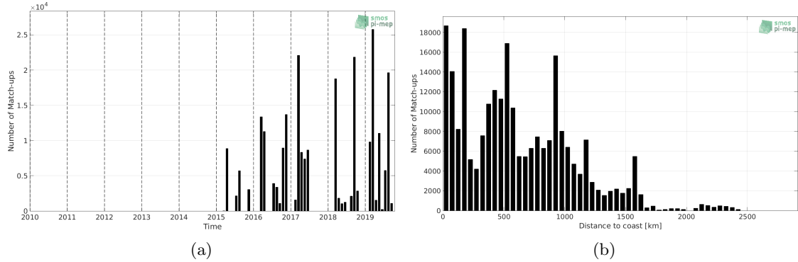
Figure 1: Number of match-ups between TSG (GOSUD-Research-vessel) and SMAP SSS L2 v4 (RSS) SSS as a function of time (a) and as function of the distance to coast (b) over the Equatorial Ocean 10N-10S Pi-MEP region and for the full satellite product period.
