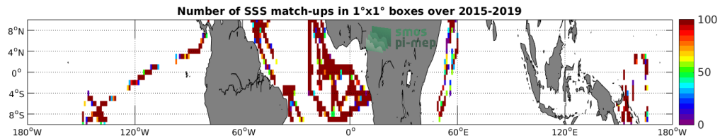
Figure 4: Number of SSS match-ups between TSG (GOSUD-Research-vessel) SSS and the SMAP SSS L2 v4 (RSS) SSS product for the Equatorial Ocean 10N-10S Pi-MEP region over 1^\circ \times 1^\circ boxes and for the full satellite product period.
