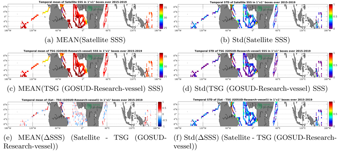
Figure 6: Temporal mean (left) and Std (right) of SSS from SMAP SSS L2 v4 (RSS) (top), TSG (GOSUD-Research-vessel) (middle), and of \Delta SSS (Satellite - TSG (GOSUD-Research-vessel)). Only match-up pairs are used to generate these maps.
