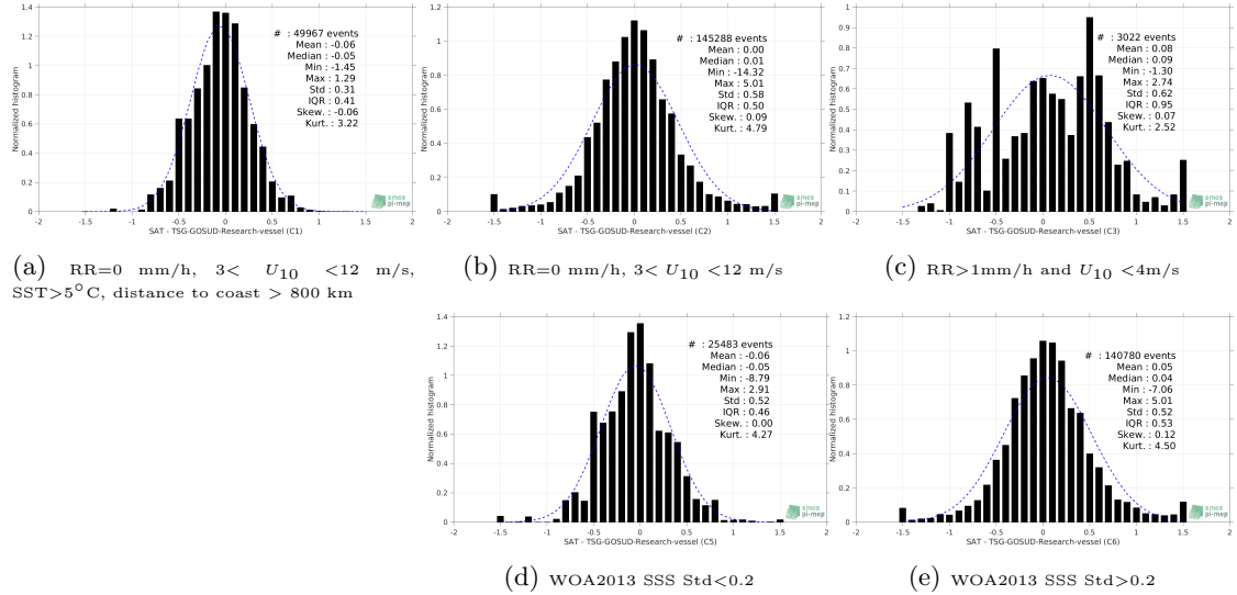
Figure 13: Normalized histogram of \Delta SSS (SMAP-L2-RSS-V4 - TSG-GOSUD-Research-vessel) for 5 different subdatasets corresponding to: RR=0 mm/h, 3 < U_{10} < 12 m/s, SST >5^\circ\text{C} , distance to coast > 800 km (a), RR=0 mm/h, 3 < U_{10} < 12 m/s (b), RR >1 mm/h and U_{10} < 4 m/s (c), WOA2013 SSS Std <0.2 (d), WOA2013 SSS Std >0.2 (e).
