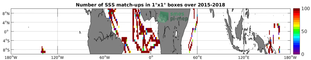
Figure 4: Number of SSS match-ups between TSG-GOSUD-Research-vessel SSS and the SMAP-L2-RSS-V4 SSS product for the Equatorial Ocean 10N-10S Pi-MEP region over 1°x1° boxes and for the full satellite product period.
