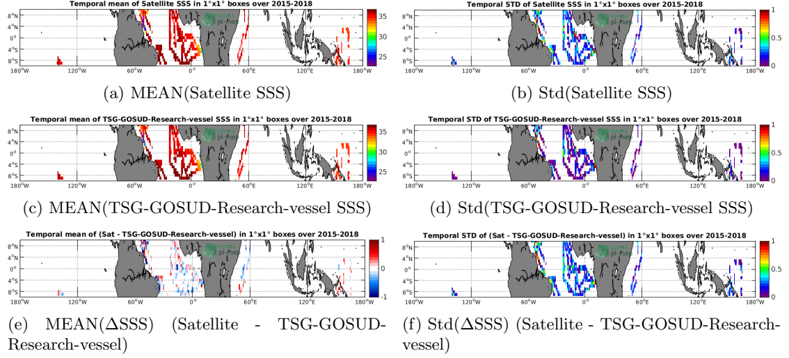
Figure 6: Temporal mean (left) and Std (right) of SSS from SMAP-L2-RSS-V4 (top), TSG-GOSUD-Research-vessel (middle), and of \Delta SSS (Satellite - TSG-GOSUD-Research-vessel). Only match-up pairs are used to generate these maps.
