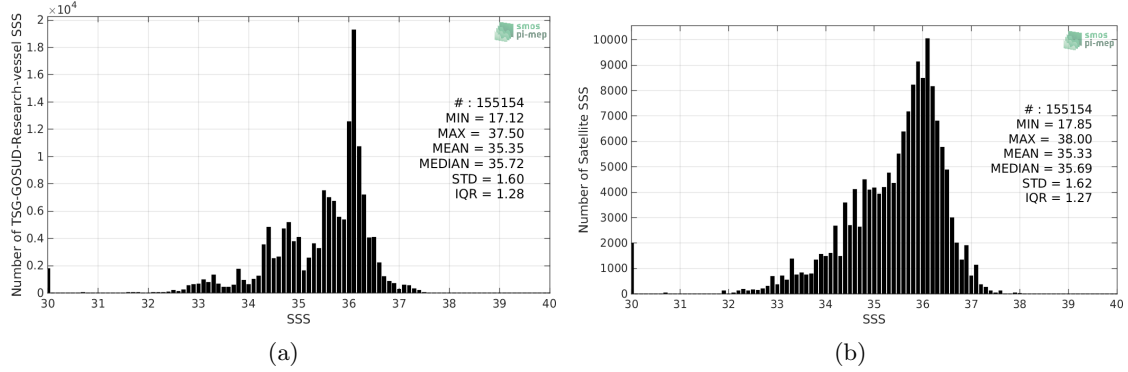
Figure 2: Histograms of SSS from TSG-GOSUD-Research-vessel (a) and SMAP-L2-RSS-V4 (b) considering all match-up pairs per bins of 0.1 over the Equatorial Ocean 10N-10S Pi-MEP region and for the full satellite product period.
