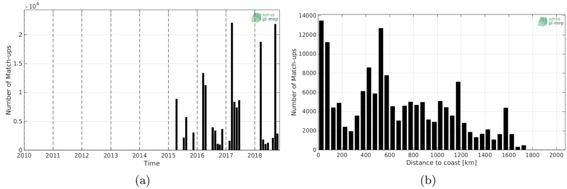
Figure 1: Number of match-ups between TSG-GOSUD-Research-vessel and SMAP-L2-RSS-V4 SSS as a function of time (a) and as function of the distance to coast (b) over the Equatorial Ocean 10N-10S Pi-MEP region and for the full satellite product period.
