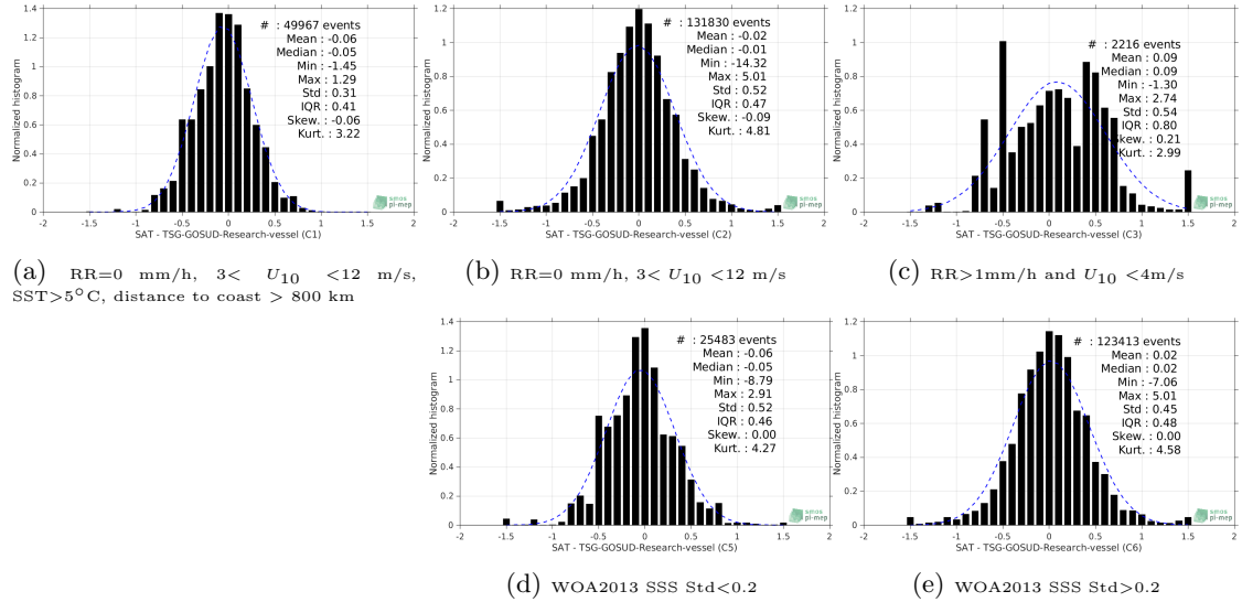
Figure 13: Normalized histogram of \Delta SSS (SMAP-L2-RSS-V4 - TSG-GOSUD-Research-vessel) for 5 different subdatasets corresponding to: RR=0 mm/h, 3 < U_{10} < 12 m/s, SST >5^\circ C, distance to coast > 800 km (a), RR=0 mm/h, 3 < U_{10} < 12 m/s (b), RR>1 mm/h and U_{10} < 4 m/s (c), WOA2013 SSS Std <0.2 (d), WOA2013 SSS Std >0.2 (e).
