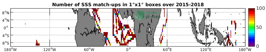
Figure 4: Number of SSS match-ups between TSG-GOSUD-Research-vessel SSS and the SMAP-L2-RSS-V4 SSS product for the Equatorial Ocean 10N-10S Pi-MEP region over 1°x1° boxes and for the full satellite product period.
