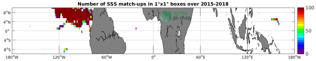
Figure 3: Number of SSS match-ups between Surface drifters SSS and the SMAP SSS L2 v4 (RSS) SSS product for the Equatorial Ocean 10N-10S Pi-MEP region over 1°x1° boxes and for the full satellite product period.
