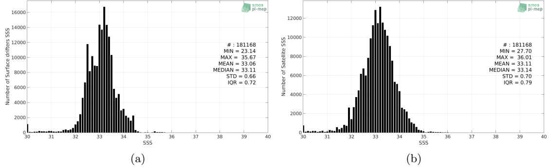
Figure 2: Histograms of SSS from Surface drifters (a) and SMAP SSS L2 v4 (RSS) (b) considering all match-up pairs per bins of 0.1 over the Equatorial Ocean 10N-10S Pi-MEP region and for the full satellite product period.
