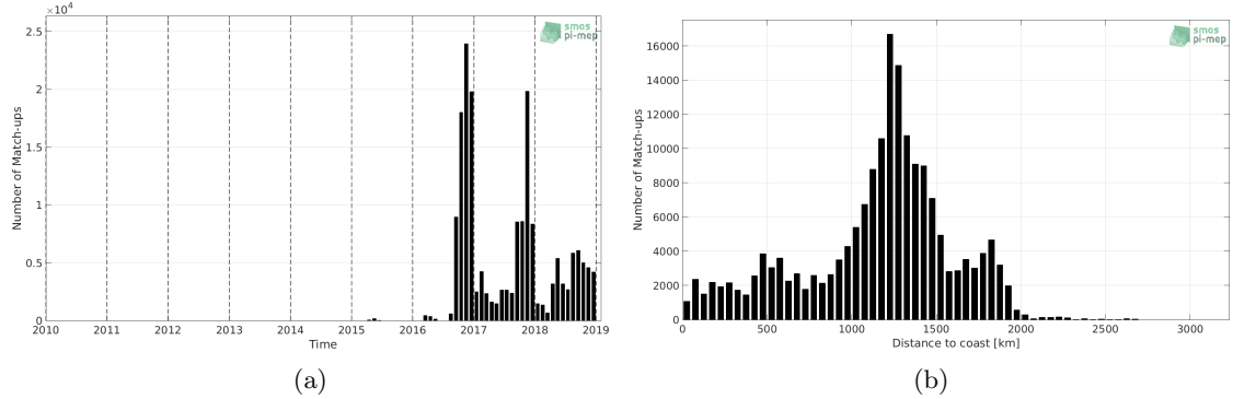
Figure 1: Number of match-ups between Surface drifters and SMAP SSS L2 v4 (RSS) SSS as a function of time (a) and as function of the distance to coast (b) over the Equatorial Ocean 10N-10S Pi-MEP region and for the full satellite product period.
