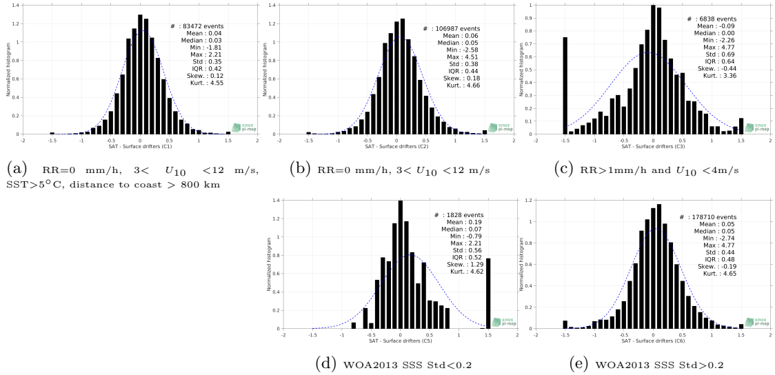
Figure 12: Normalized histogram of \Delta SSS (SMAP SSS L2 v4 (RSS) - Surface drifters) for 5 different subdatasets corresponding to: RR=0 mm/h, 3 < U_{10} < 12 m/s, SST >5^\circ C, distance to coast > 800 km (a), RR=0 mm/h, 3 < U_{10} < 12 m/s (b), RR>1 mm/h and U_{10} < 4 m/s (c), WOA2013 SSS Std <0.2 (d), WOA2013 SSS Std >0.2 (e).
