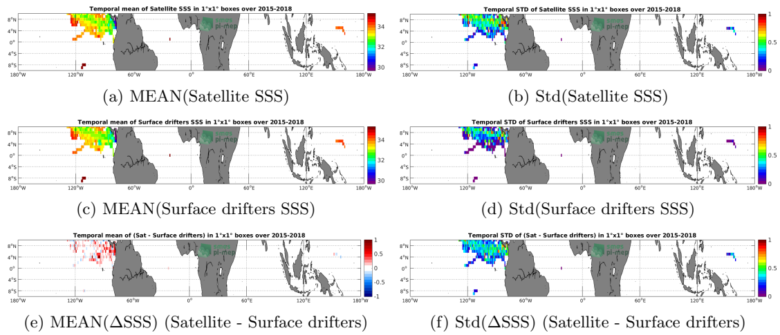
Figure 5: Temporal mean (left) and Std (right) of SSS from SMAP-L2-RSS-V4 (top), Surface drifters (middle), and of \Delta SSS (Satellite - Surface drifters). Only match-up pairs are used to generate these maps.
