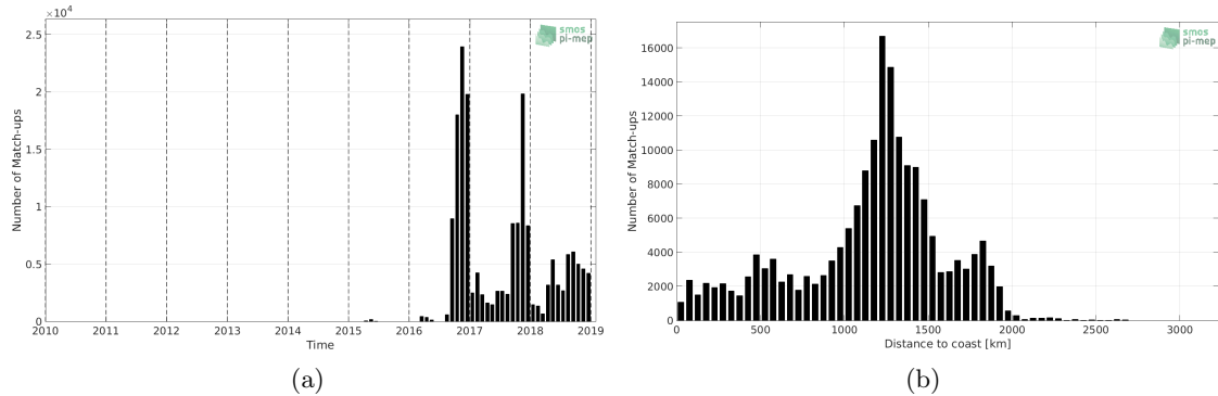
Figure 1: Number of match-ups between Surface drifters and SMAP-L2-RSS-V4 SSS as a function of time (a) and as function of the distance to coast (b) over the Equatorial Ocean 10N-10S Pi-MEP region and for the full satellite product period.
