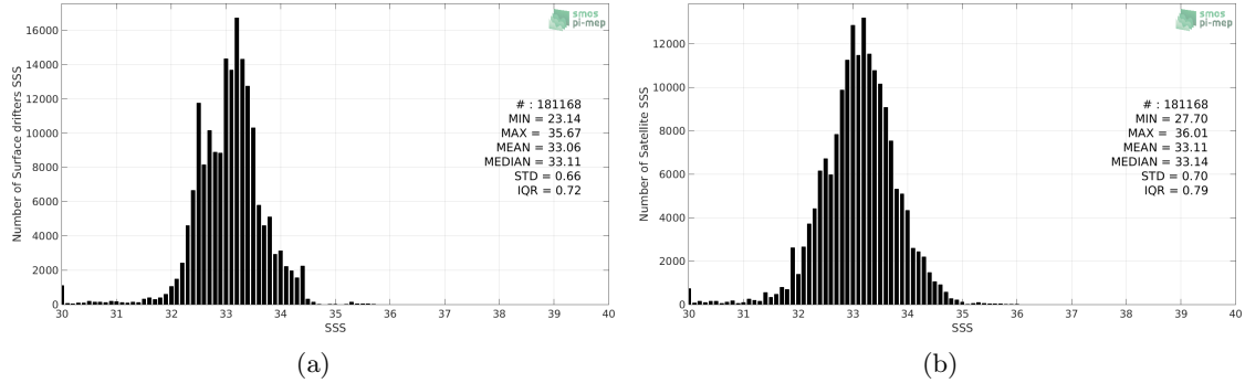
Figure 2: Histograms of SSS from Surface drifters (a) and SMAP-L2-RSS-V4 (b) considering all match-up pairs per bins of 0.1 over the Equatorial Ocean 10N-10S Pi-MEP region and for the full satellite product period.
