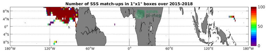
Figure 3: Number of SSS match-ups between Surface drifters SSS and the SMAP-L2-RSS-V4 SSS product for the Equatorial Ocean 10N-10S Pi-MEP region over 1°x1° boxes and for the full satellite product period.
