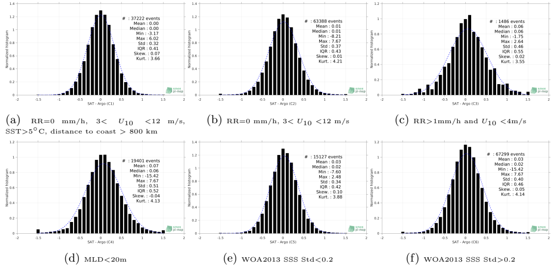
Figure 13: Normalized histogram of \Delta SSS (SMAP SSS L2 v4 (RSS) - Argo) for 6 different subdatasets corresponding to: RR=0 mm/h, 3 < U_{10} < 12 m/s, SST >5^\circ\text{C} , distance to coast > 800 km (a), RR=0 mm/h, 3 < U_{10} < 12 m/s (b), RR >1 mm/h and U_{10} < 4 m/s (c), MLD <20 m (d), WOA2013 SSS Std <0.2 (e), WOA2013 SSS Std >0.2 (f).
