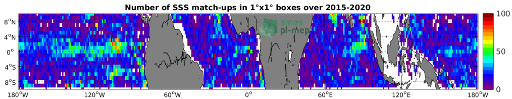
Figure 4: Number of SSS match-ups between Argo SSS and the SMAP SSS L2 v4 (RSS) SSS product for the Equatorial Ocean 10N-10S Pi-MEP region over 1°x1° boxes and for the full satellite product period.
