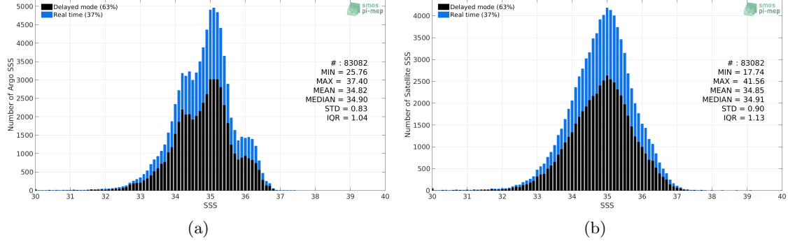
Figure 2: Histograms of SSS from Argo (a) and SMAP SSS L2 v4 (RSS) (b) considering all match-up pairs per bins of 0.1 over the Equatorial Ocean 10N-10S Pi-MEP region and for the full satellite product period.
