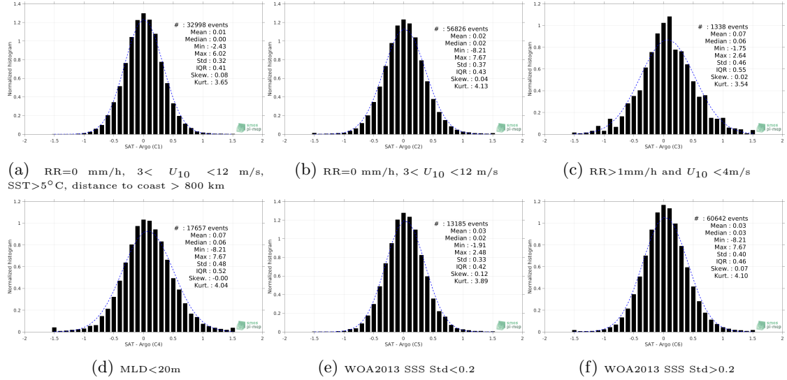
Figure 13: Normalized histogram of \Delta SSS (SMAP-L2-RSS-V4 - Argo) for 6 different subdatasets corresponding to: RR=0 mm/h, 3 < U_{10} < 12 m/s, SST >5^\circ\text{C} , distance to coast > 800 km (a), RR=0 mm/h, 3 < U_{10} < 12 m/s (b), RR >1 mm/h and U_{10} < 4 m/s (c), MLD <20 m (d), WOA2013 SSS Std <0.2 (e), WOA2013 SSS Std >0.2 (f).
