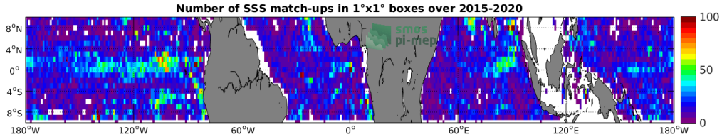
Figure 4: Number of SSS match-ups between Argo SSS and the SMAP-L2-RSS-V4 SSS product for the Equatorial Ocean 10N-10S Pi-MEP region over 1°x1° boxes and for the full satellite product period.
