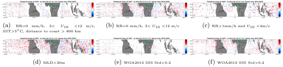
Figure 12: Temporal mean gridded over spatial boxes of size 1^\circ \times 1^\circ of \Delta SSS (SMAP-L2-RSS-V4 - Argo) for 6 different subdatasets corresponding to: RR=0 mm/h, 3 < U_{10} < 12 m/s, SST >5^\circ\text{C} , distance to coast > 800 km (a), RR=0 mm/h, 3 < U_{10} < 12 m/s (b), RR >1 mm/h and U_{10} < 4 m/s (c),MLD <20 m (d),WOA2013 SSS Std <0.2 (e),WOA2013 SSS Std >0.2 (f).
