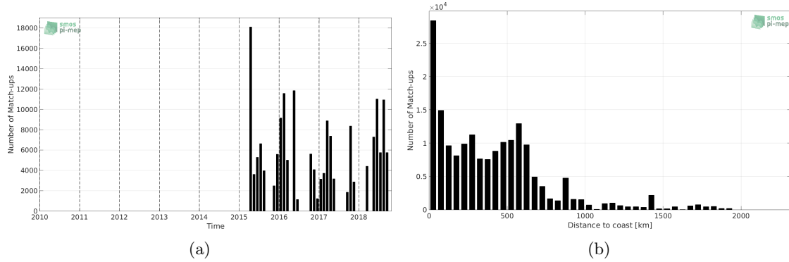
Figure 1: Number of match-ups between TSG-SAMOS and SMAP-L2-RSS-V3-70KM SSS as a function of time (a) and as function of the distance to coast (b) over the Equatorial Ocean 10N-10S Pi-MEP region and for the full satellite product period.
