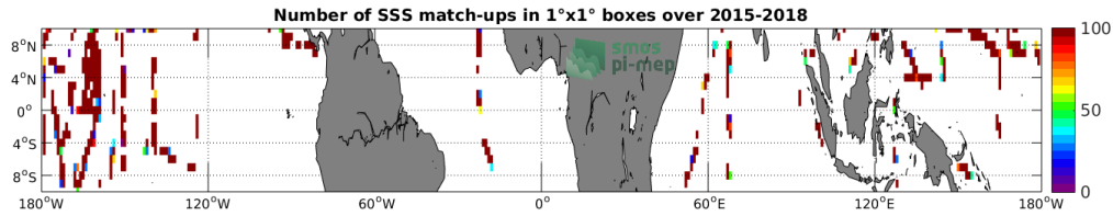
Figure 4: Number of SSS match-ups between TSG-SAMOS SSS and the SMAP-L2-RSS-V3-70KM SSS product for the Equatorial Ocean 10N-10S Pi-MEP region over 1°x1° boxes and for the full satellite product period.
