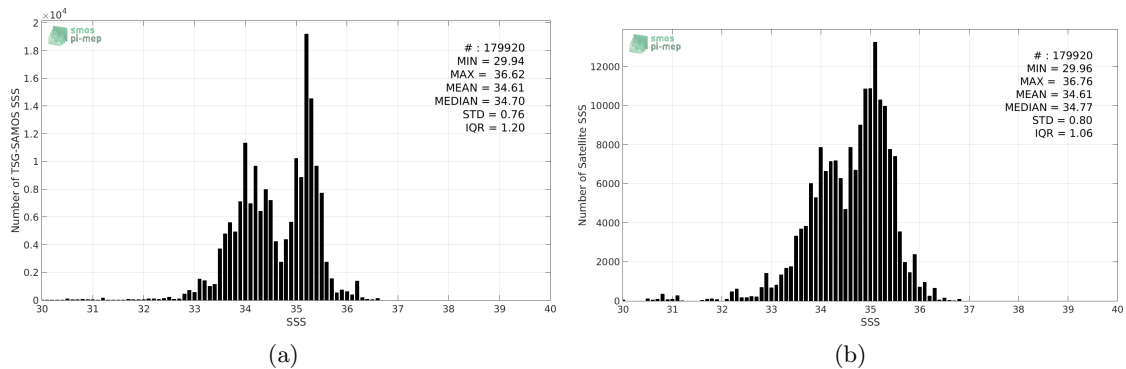
Figure 2: Histograms of SSS from TSG-SAMOS (a) and SMAP-L2-RSS-V3-70KM (b) considering all match-up pairs per bins of 0.1 over the Equatorial Ocean 10N-10S Pi-MEP region and for the full satellite product period.
