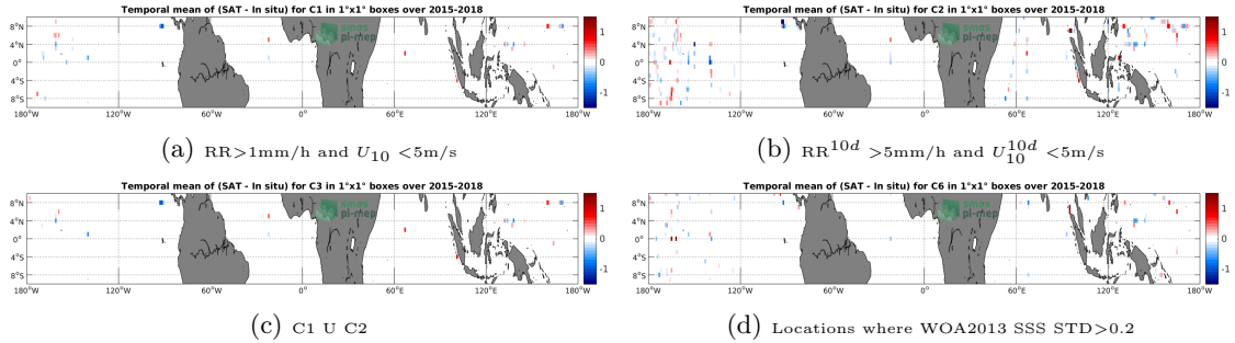
Figure 12: Temporal mean gridded over spatial boxes of size 1^\circ \times 1^\circ of \Delta SSS (SMAP-L2-RSS-V3-70KM - TSG-SAMOS) for 4 different subdatasets corresponding to: RR > 1\text{mm/h} and U_{10} < 5\text{m/s} (a), RR ^{10d} > 5\text{mm/h} and U_{10}^{10d} < 5\text{m/s} (b), C1 U C2 (c), Locations where WOA2013 SSS STD > 0.2 (d).
