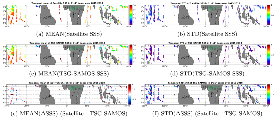
Figure 6: Temporal mean (left) and STD (right) of SSS from SMAP-L2-RSS-V3-70KM (top), TSG-SAMOS (middle), and of \Delta SSS (Satellite - TSG-SAMOS). Only match-up pairs are used to generate these maps.
