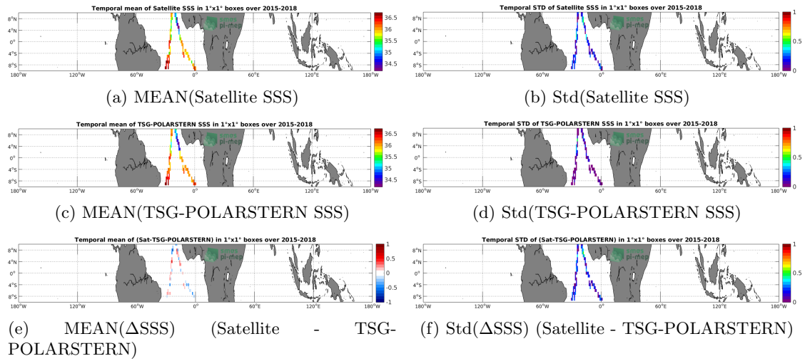
Figure 6: Temporal mean (left) and Std (right) of SSS from SMAP-L2-RSS-V3-70KM (top), TSG-POLARSTERN (middle), and of \Delta SSS (Satellite - TSG-POLARSTERN). Only match-up pairs are used to generate these maps.
