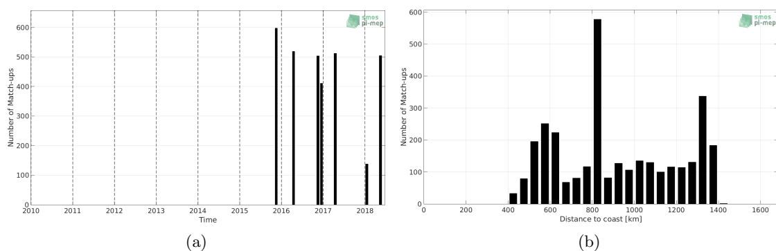
Figure 1: Number of match-ups between TSG-POLARSTERN and SMAP-L2-RSS-V3-70KM SSS as a function of time (a) and as function of the distance to coast (b) over the Equatorial Ocean 10N-10S Pi-MEP region and for the full satellite product period.
