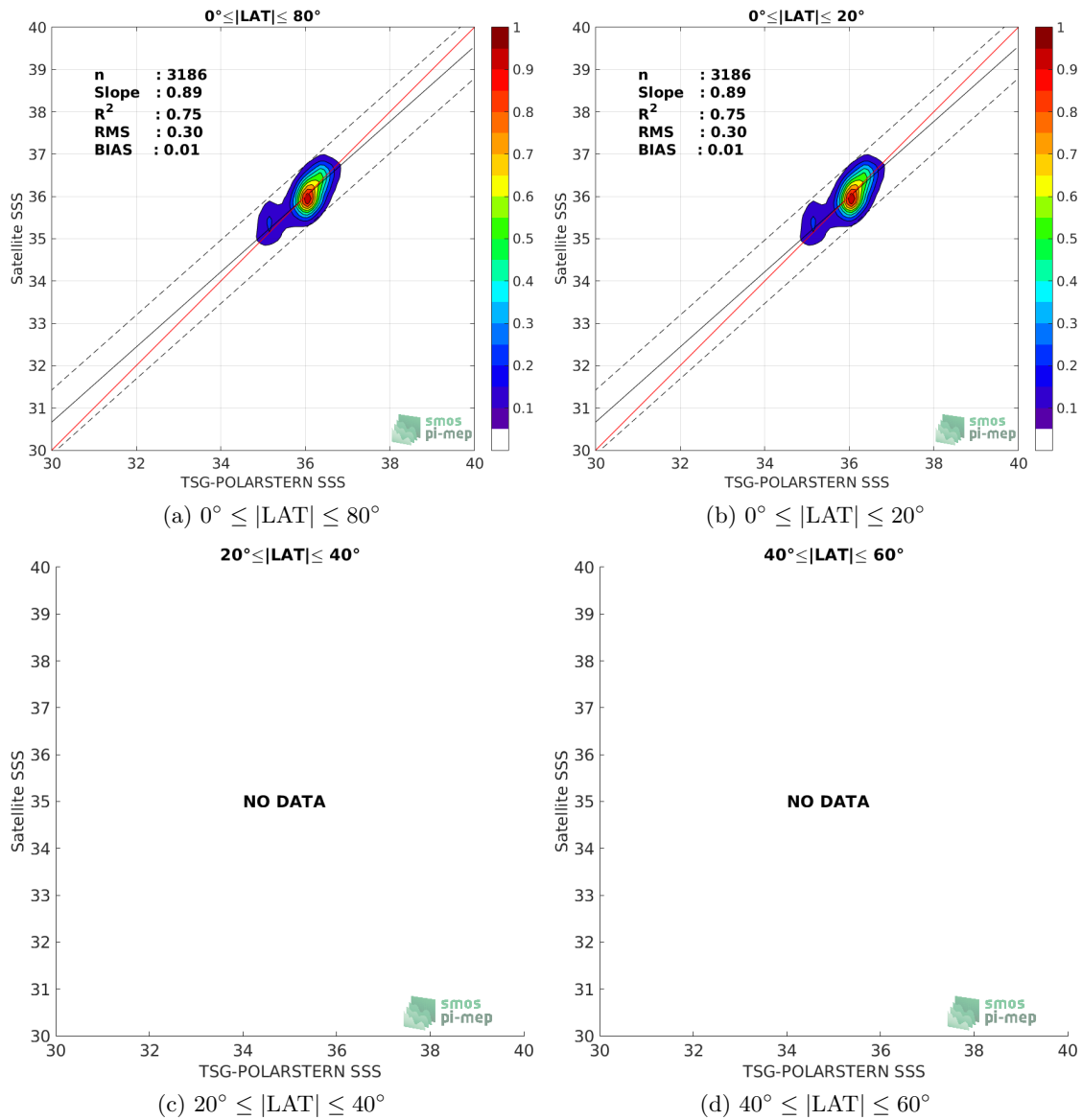
Figure 9: Contour maps of the concentration of SMAP-L2-RSS-V3-70KM SSS (y-axis) versus TSG-POLARSTERN SSS (x-axis) at match-up pairs for different latitude bands. For each plot, the red line shows x=y . The black thin and dashed lines indicate a linear fit through the data cloud and the \pm 95\% confidence levels, respectively. The number match-up pairs n , the slope and R^2 coefficient of the linear fit, the root mean square (RMS) and the mean bias between satellite and in situ data are indicated for each latitude band in each plots.
