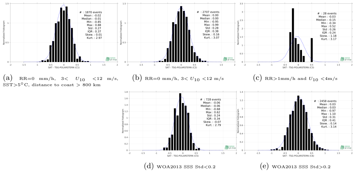
Figure 13: Normalized histogram of \Delta SSS (SMAP-L2-RSS-V3-70KM - TSG-POLARSTERN) for 5 different subdatasets corresponding to: RR=0 mm/h, 3 < U_{10} < 12 m/s, SST >5^\circ C, distance to coast > 800 km (a), RR=0 mm/h, 3 < U_{10} < 12 m/s (b), RR >1 mm/h and U_{10} < 4 m/s (c), WOA2013 SSS Std <0.2 (d), WOA2013 SSS Std >0.2 (e).
