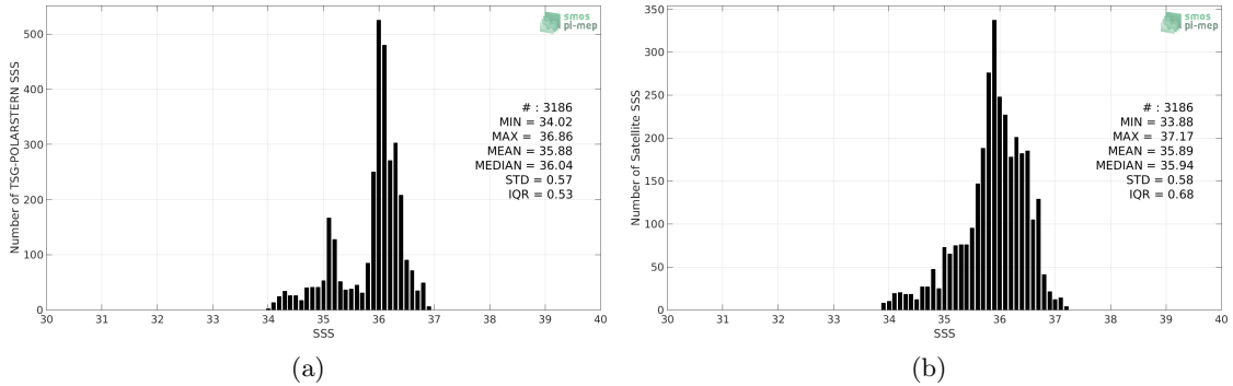
Figure 2: Histograms of SSS from TSG-POLARSTERN (a) and SMAP-L2-RSS-V3-70KM (b) considering all match-up pairs per bins of 0.1 over the Equatorial Ocean 10N-10S Pi-MEP region and for the full satellite product period.
