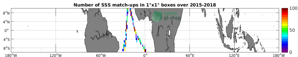
Figure 4: Number of SSS match-ups between TSG-POLARSTERN SSS and the SMAP-L2-RSS-V3-70KM SSS product for the Equatorial Ocean 10N-10S Pi-MEP region over 1^\circ \times 1^\circ boxes and for the full satellite product period.
