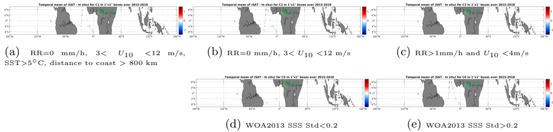
Figure 12: Temporal mean gridded over spatial boxes of size 1^\circ \times 1^\circ of \Delta SSS (SMAP-L2-RSS-V3-70KM - TSG-POLARSTERN) for 5 different subdatasets corresponding to:RR=0 mm/h, 3 < U_{10} < 12 m/s, SST >5^\circ C, distance to coast > 800 km (a), RR=0 mm/h, 3 < U_{10} < 12 m/s (b), RR >1 mm/h and U_{10} < 4 m/s (c), WOA2013 SSS Std <0.2 (d), WOA2013 SSS Std >0.2 (e).
