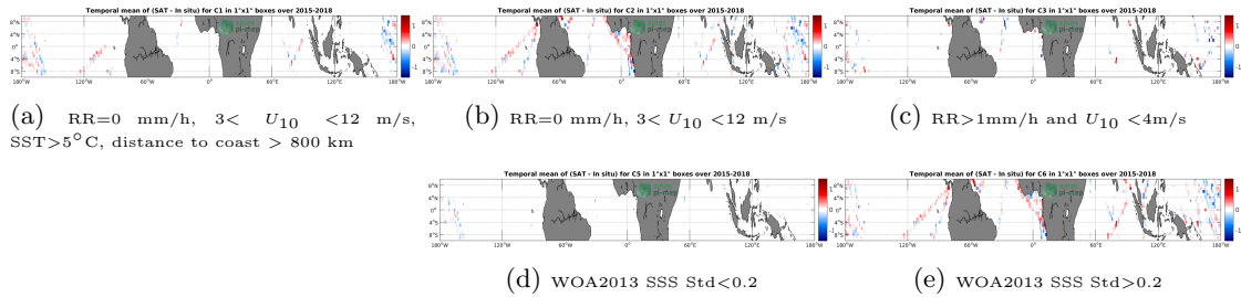
Figure 12: Temporal mean gridded over spatial boxes of size 1^\circ \times 1^\circ of \Delta SSS (SMAP-L2-RSS-V3-70KM - TSG-LEGOS-DM) for 5 different subdatasets corresponding to:RR=0 mm/h, 3 < U_{10} < 12 m/s, SST > 5^\circ C , distance to coast > 800 km (a), RR=0 mm/h, 3 < U_{10} < 12 m/s (b), RR >1 mm/h and U_{10} < 4 m/s (c), WOA2013 SSS Std <0.2 (d), WOA2013 SSS Std >0.2 (e).
