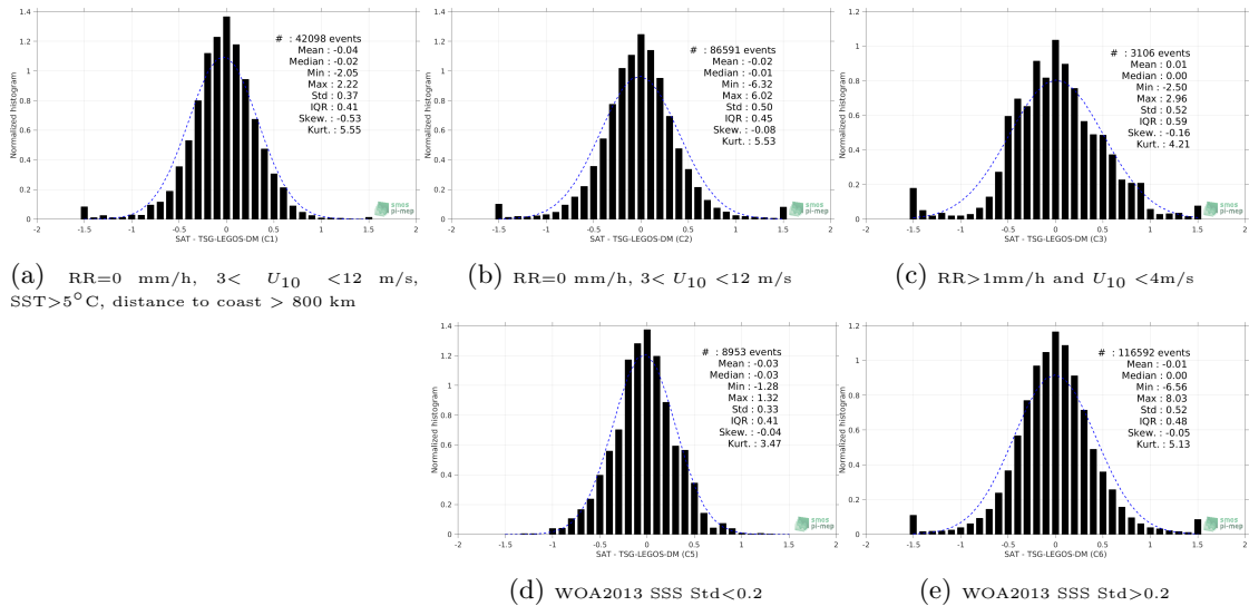
Figure 13: Normalized histogram of \Delta SSS (SMAP-L2-RSS-V3-70KM - TSG-LEGOS-DM) for 5 different subdatasets corresponding to: RR=0 mm/h, 3 < U_{10} < 12 m/s, SST > 5^\circ C , distance to coast > 800 km (a), RR=0 mm/h, 3 < U_{10} < 12 m/s (b), RR >1 mm/h and U_{10} < 4 m/s (c), WOA2013 SSS Std <0.2 (d), WOA2013 SSS Std >0.2 (e).
