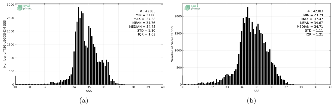
Figure 2: Histograms of SSS from TSG-LEGOS-DM (a) and SMAP-L2-RSS-V3-70KM (b) considering all match-up pairs per bins of 0.1 over the Equatorial Ocean 10N-10S Pi-MEP region and for the full satellite product period.
