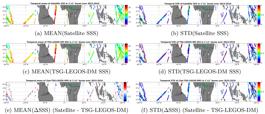
Figure 6: Temporal mean (left) and STD (right) of SSS from SMAP-L2-RSS-V3-70KM (top), TSG-LEGOS-DM (middle), and of \Delta SSS (Satellite - TSG-LEGOS-DM). Only match-up pairs are used to generate these maps.
