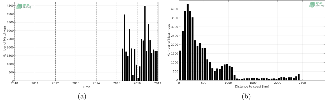
Figure 1: Number of match-ups between TSG-LEGOS-DM and SMAP-L2-RSS-V3-70KM SSS as a function of time (a) and as function of the distance to coast (b) over the Equatorial Ocean 10N-10S Pi-MEP region and for the full satellite product period.
