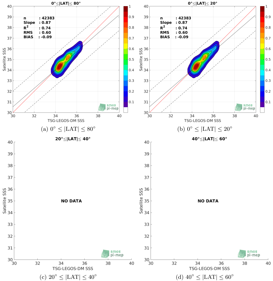
Figure 9: Contour maps of the concentration of SMAP-L2-RSS-V3-70KM SSS (y-axis) versus TSG-LEGOS-DM SSS (x-axis) at match-up pairs for different latitude bands. For each plot, the red line shows x=y . The black thin and dashed lines indicate a linear fit through the data cloud and the \pm 95\% confidence levels, respectively. The number match-up pairs n , the slope and R^2 coefficient of the linear fit, the root mean square (RMS) and the mean bias between satellite and in situ data are indicated for each latitude band in each plots.
