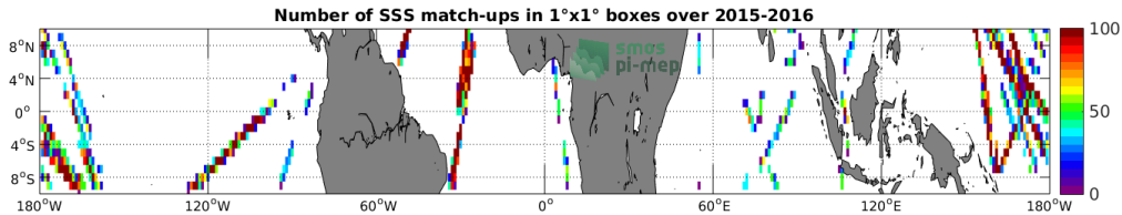
Figure 4: Number of SSS match-ups between TSG-LEGOS-DM SSS and the SMAP-L2-RSS-V3-70KM SSS product for the Equatorial Ocean 10N-10S Pi-MEP region over 1^\circ \times 1^\circ boxes and for the full satellite product period.
