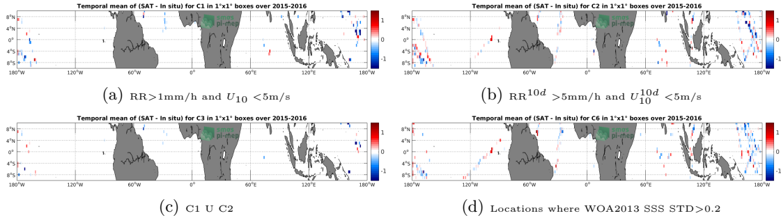
Figure 12: Temporal mean gridded over spatial boxes of size 1^\circ \times 1^\circ of \Delta SSS (SMAP-L2-RSS-V3-70KM - TSG-LEGOS-DM) for 4 different subdatasets corresponding to: RR > 1\text{mm/h} and U_{10} < 5\text{m/s} (a), RR^{10d} > 5\text{mm/h} and U_{10}^{10d} < 5\text{m/s} (b), C1 U C2 (c), Locations where WOA2013 SSS STD > 0.2 (d).
