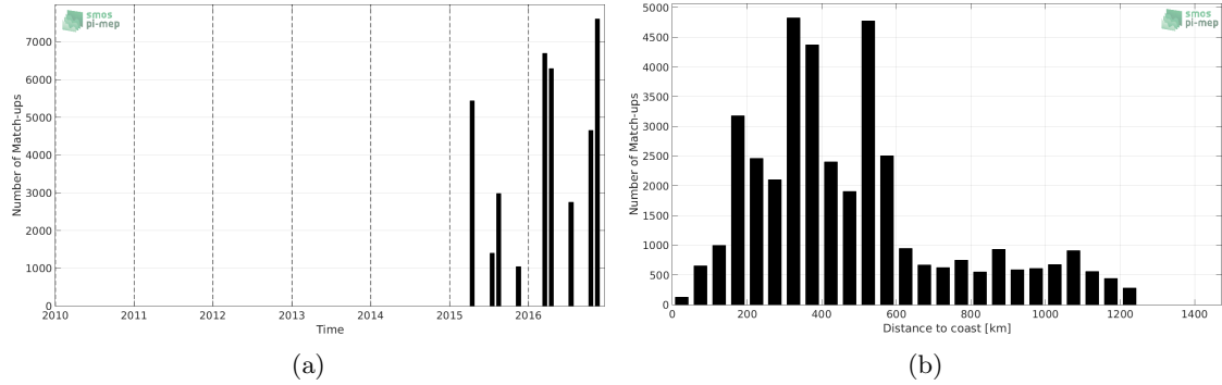
Figure 1: Number of match-ups between TSG-GOSUD-Research-vessel and SMAP-L2-RSS-V3-70KM SSS as a function of time (a) and as function of the distance to coast (b) over the Equatorial Ocean 10N-10S Pi-MEP region and for the full satellite product period.
