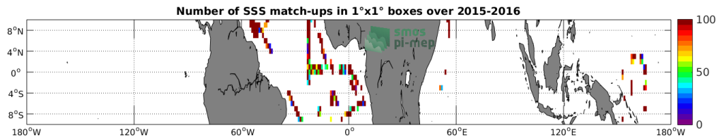
Figure 4: Number of SSS match-ups between TSG-GOSUD-Research-vessel SSS and the SMAP-L2-RSS-V3-70KM SSS product for the Equatorial Ocean 10N-10S Pi-MEP region over 1^\circ \times 1^\circ boxes and for the full satellite product period.
