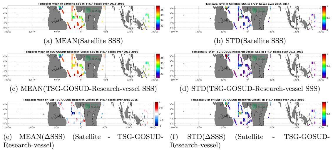
Figure 6: Temporal mean (left) and STD (right) of SSS from SMAP-L2-RSS-V3-70KM (top), TSG-GOSUD-Research-vessel (middle), and of \Delta SSS (Satellite - TSG-GOSUD-Research-vessel). Only match-up pairs are used to generate these maps.
