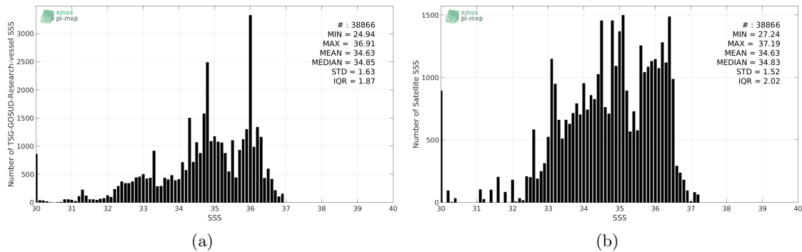
Figure 2: Histograms of SSS from TSG-GOSUD-Research-vessel (a) and SMAP-L2-RSS-V3-70KM (b) considering all match-up pairs per bins of 0.1 over the Equatorial Ocean 10N-10S Pi-MEP region and for the full satellite product period.
