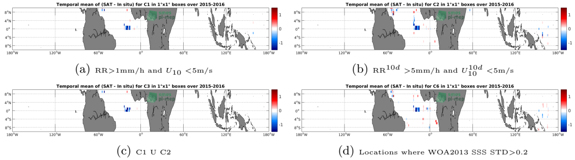
Figure 12: Temporal mean gridded over spatial boxes of size 1^\circ \times 1^\circ of \Delta SSS (SMAP-L2-RSS-V3-70KM - TSG-GOSUD-Research-vessel) for 4 different subdatasets corresponding to: RR > 1\text{mm/h} and U_{10} < 5\text{m/s} (a), RR^{10d} > 5\text{mm/h} and U_{10}^{10d} < 5\text{m/s} (b), C1 U C2 (c), Locations where WOA2013 SSS STD > 0.2 (d).
