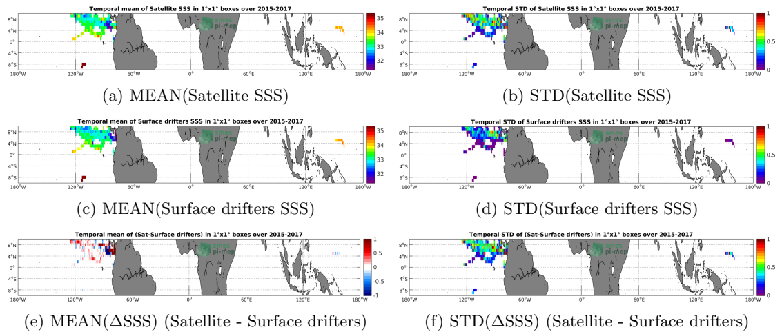
Figure 5: Temporal mean (left) and STD (right) of SSS from SMAP-L2-RSS-V3-70KM (top), Surface drifters (middle), and of \Delta SSS (Satellite - Surface drifters). Only match-up pairs are used to generate these maps.
