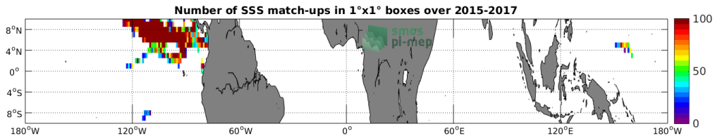
Figure 3: Number of SSS match-ups between Surface drifters SSS and the SMAP-L2-RSS-V3-70KM SSS product for the Equatorial Ocean 10N-10S Pi-MEP region over 1°x1° boxes and for the full satellite product period.
