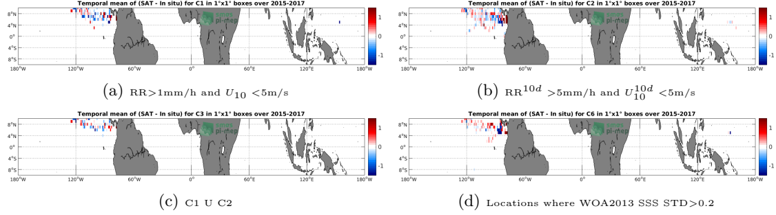
Figure 11: Temporal mean gridded over spatial boxes of size 1^\circ \times 1^\circ of \Delta SSS (SMAP-L2-RSS-V3-70KM - Surface drifters) for 4 different subdatasets corresponding to: RR > 1\text{mm/h} and U_{10} < 5\text{m/s} (a), RR^{10d} > 5\text{mm/h} and U_{10}^{10d} < 5\text{m/s} (b), C1 U C2 (c), Locations where WOA2013 SSS STD > 0.2 (d).
