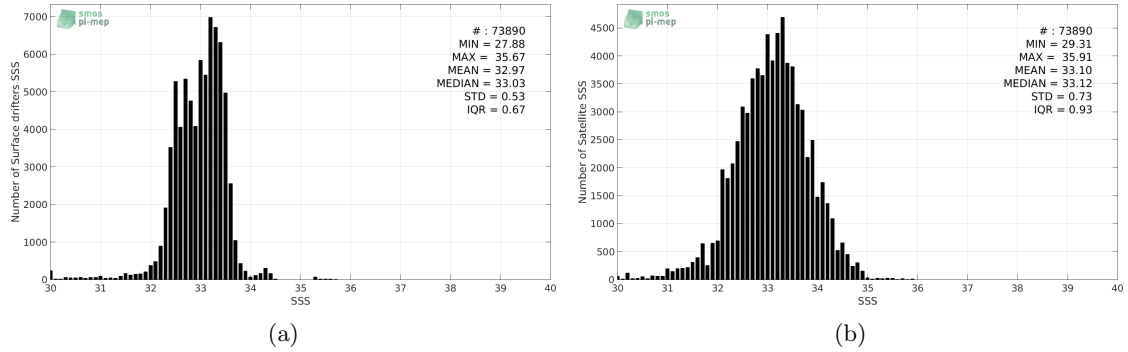
Figure 2: Histograms of SSS from Surface drifters (a) and SMAP-L2-RSS-V3-70KM (b) considering all match-up pairs per bins of 0.1 over the Equatorial Ocean 10N-10S Pi-MEP region and for the full satellite product period.
