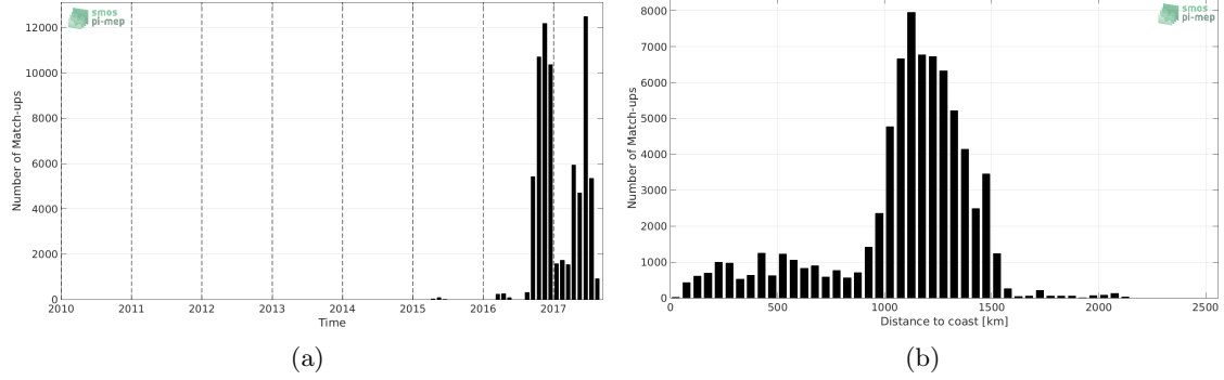
Figure 1: Number of match-ups between Surface drifters and SMAP-L2-RSS-V3-70KM SSS as a function of time (a) and as function of the distance to coast (b) over the Equatorial Ocean 10N-10S Pi-MEP region and for the full satellite product period.
