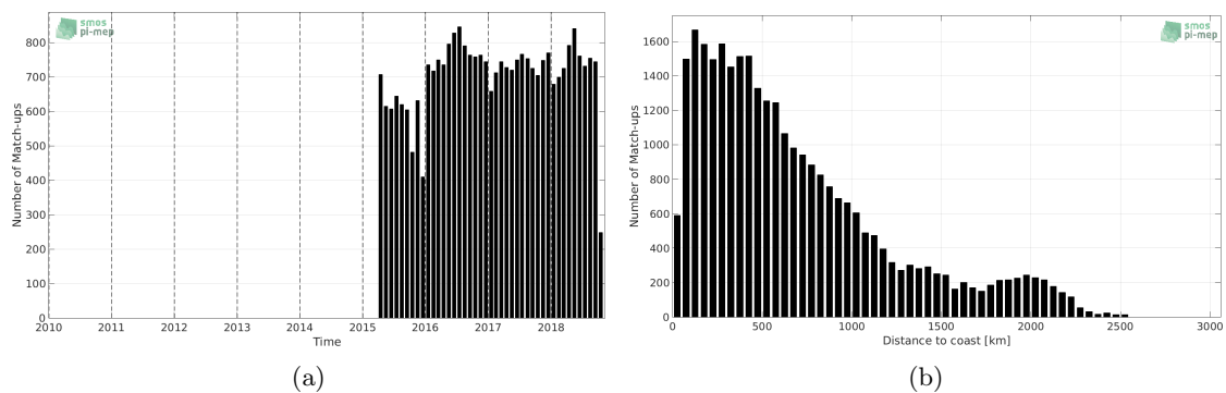
Figure 1: Number of match-ups between Argo and SMAP-L2-RSS-V3-70KM SSS as a function of time (a) and as function of the distance to coast (b) over the Equatorial Ocean 10N-10S Pi-MEP region and for the full satellite product period.
