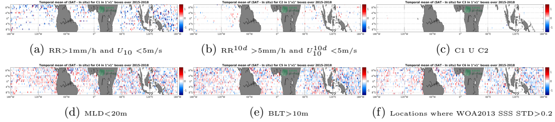
Figure 12: Temporal mean gridded over spatial boxes of size 1^\circ \times 1^\circ of \Delta\text{SSS} (SMAP-L2-RSS-V3-70KM - Argo) for 6 different subdatasets corresponding to: \text{RR} > 1\text{mm/h} and U_{10} < 5\text{m/s} (a), \text{RR}^{10d} > 5\text{mm/h} and U_{10}^{10d} < 5\text{m/s} (b), C1 U C2 (c), \text{MLD} < 20\text{m} (d), \text{BLT} > 10\text{m} (e), Locations where WOA2013 SSS \text{STD} > 0.2 (f).
