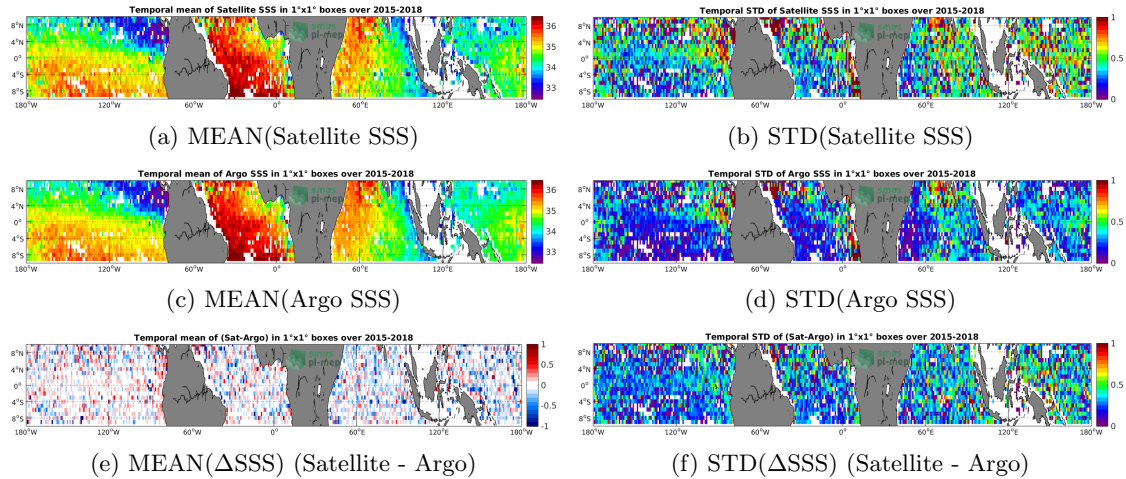
Figure 6: Temporal mean (left) and STD (right) of SSS from SMAP-L2-RSS-V3-70KM (top), Argo (middle), and of \Delta SSS (Satellite - Argo). Only match-up pairs are used to generate these maps.
