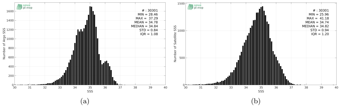
Figure 2: Histograms of SSS from Argo (a) and SMAP-L2-RSS-V3-70KM (b) considering all match-up pairs per bins of 0.1 over the Equatorial Ocean 10N-10S Pi-MEP region and for the full satellite product period.
