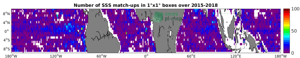
Figure 4: Number of SSS match-ups between Argo SSS and the SMAP-L2-RSS-V3-70KM SSS product for the Equatorial Ocean 10N-10S Pi-MEP region over 1^\circ \times 1^\circ boxes and for the full satellite product period.
