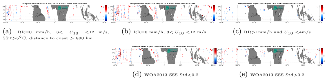
Figure 14: Temporal mean gridded over spatial boxes of size 1^\circ \times 1^\circ of \Delta SSS (SMAP SSS L2 v5.0 (JPL) - TSG (SAMOS)) for 5 different subdatasets corresponding to:RR=0 mm/h, 3 < U_{10} < 12 m/s, SST>5°C, distance to coast > 800 km (a), RR=0 mm/h, 3 < U_{10} < 12 m/s (b), RR>1mm/h and U_{10} < 4 m/s (c), WOA2013 SSS Std<0.2 (d), WOA2013 SSS Std>0.2 (e).
