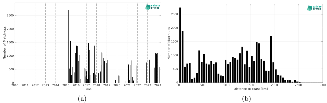
Figure 2: Number of match-ups between TSG (SAMOS) and SMAP SSS L2 v5.0 (JPL) SSS as a function of time (a) and as function of the distance to coast (b) over the Equatorial Ocean 10N-10S Pi-MEP region and for the full satellite product period.
