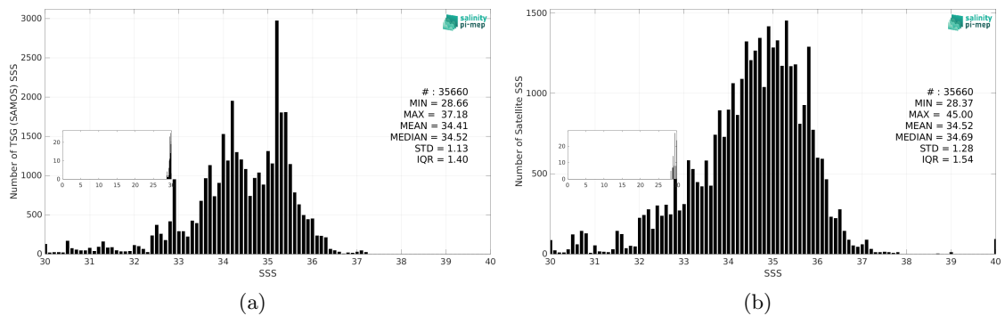
Figure 3: Histograms of SSS from TSG (SAMOS) (a) and SMAP SSS L2 v5.0 (JPL) (b) considering all match-up pairs per bins of 0.1 over the Equatorial Ocean 10N-10S Pi-MEP region and for the full satellite product period.
