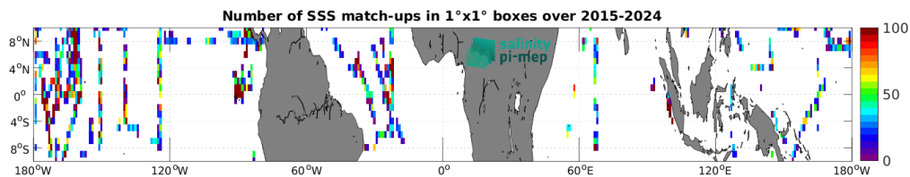
Figure 5: Number of SSS match-ups between TSG (SAMOS) SSS and the SMAP SSS L2 v5.0 (JPL) SSS product for the Equatorial Ocean 10N-10S Pi-MEP region over 1^\circ \times 1^\circ boxes and for the full satellite product period.
