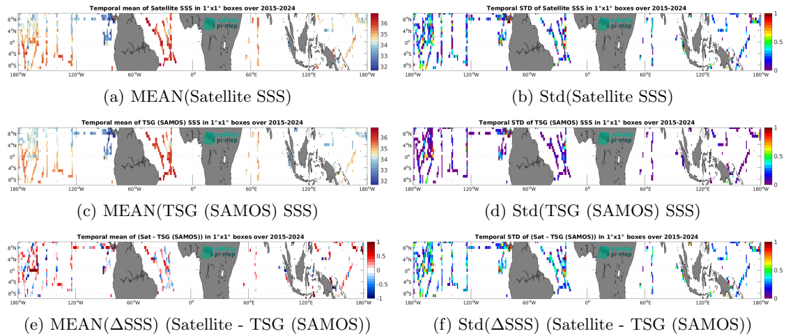
Figure 7: Temporal mean (left) and Std (right) of SSS from SMAP SSS L2 v5.0 (JPL) (top), TSG (SAMOS) (middle), and of \Delta SSS (Satellite - TSG (SAMOS)). Only match-up pairs are used to generate these maps.
